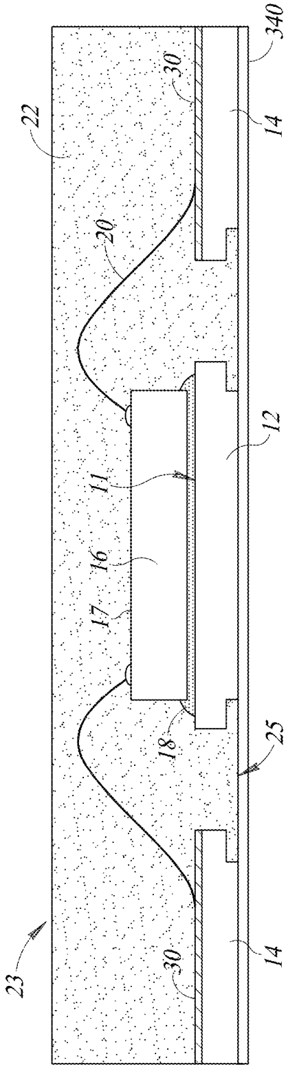
FIG. 3D
