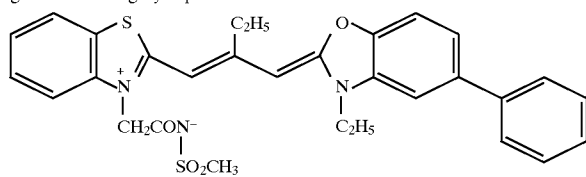
red sensitizing dye cpd 13
