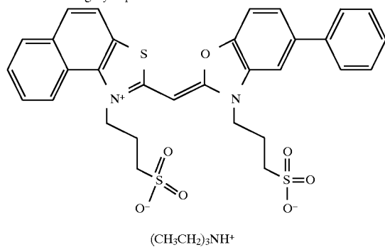
blue sensitizing dye cpd 15
