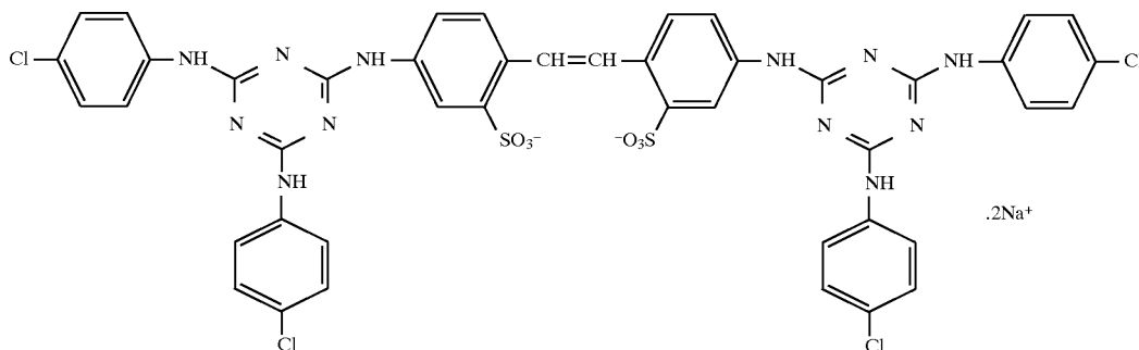
supersensitizer cpd 2
