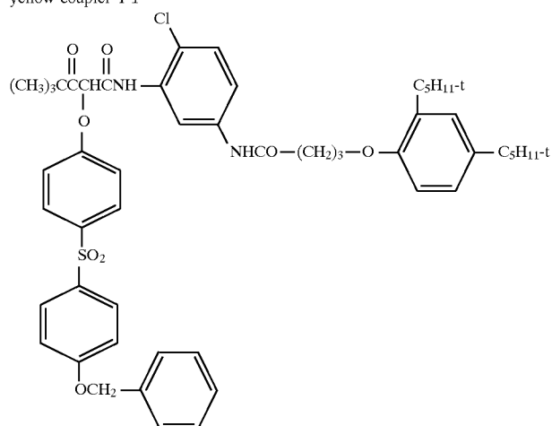
yellow dye cpd 8
