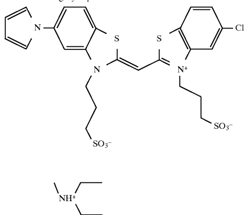
blue sensitizing dye cpd 15
