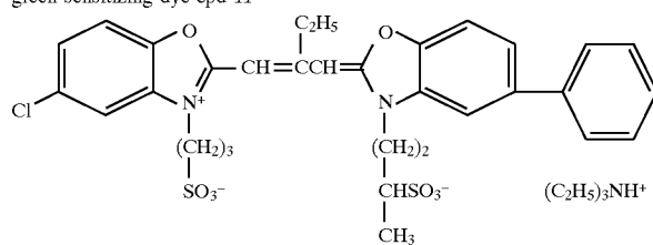
green sensitizing dye cpd 11
