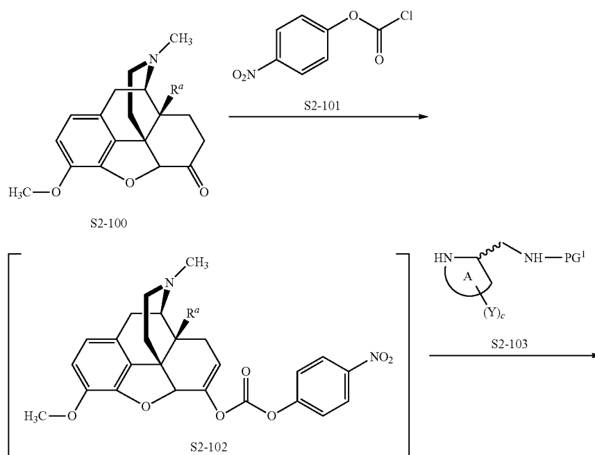
Scheme 4
