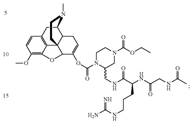
Compound KC-43:
