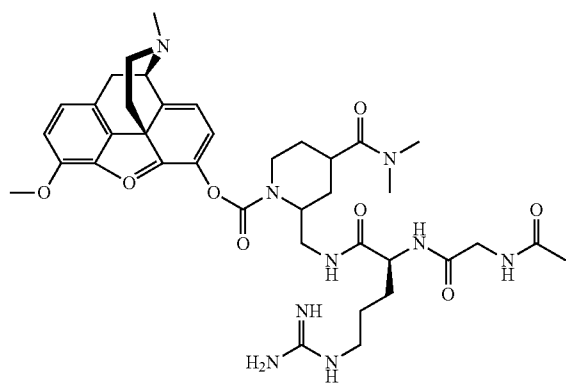
Compound KC-47:
