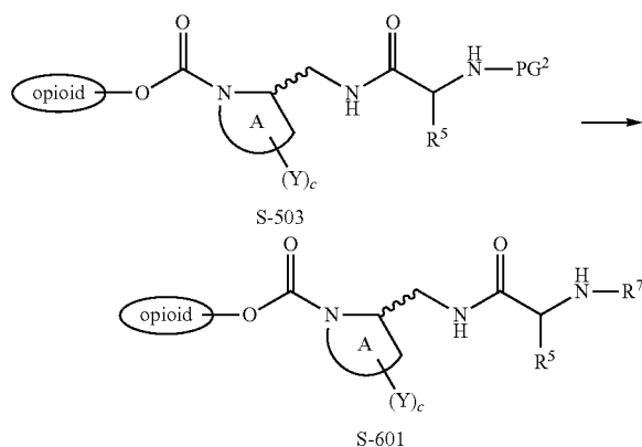
Scheme 9
