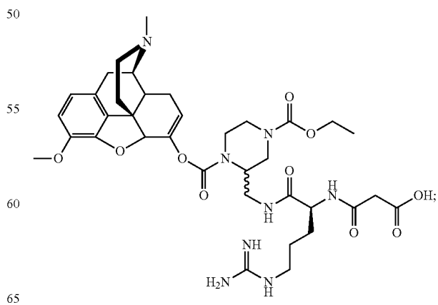
Compound KC-44:
