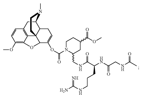
Compound KC-41:
