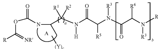
imine tautomer
