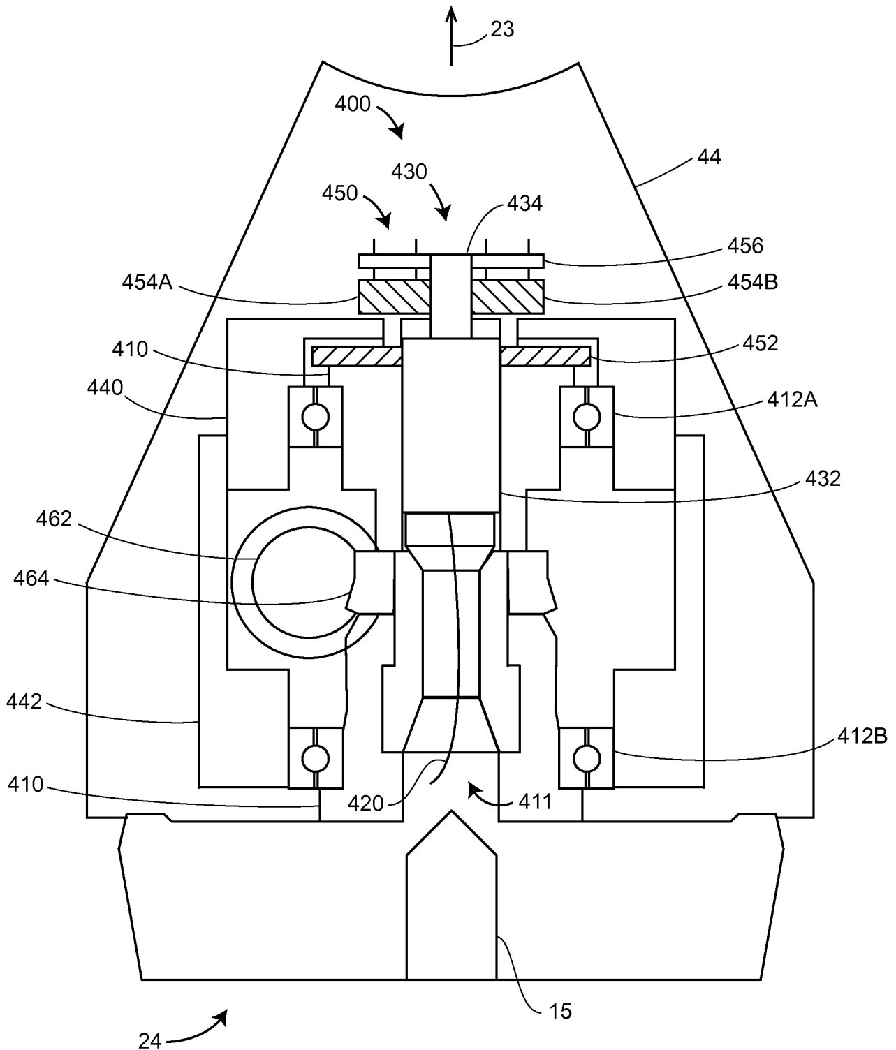
CROSS SECTION A-A FIG. 4
