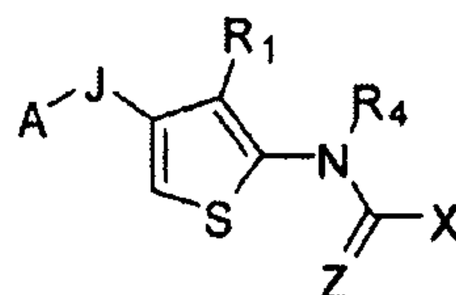
Formula (III);
