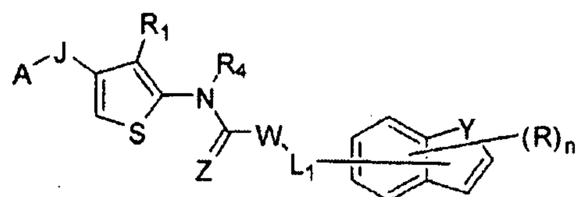
Formula (II);
