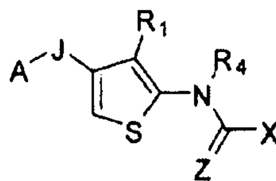
Formula (I);
