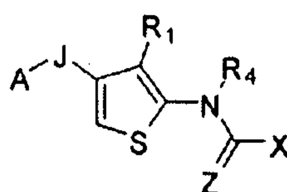
Formula (I);
