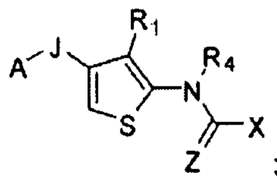
Formula (IV)
