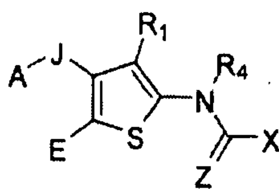
Formula (V);
