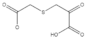
3-[(carboxymethyl)sulfanyl]-2-oxopropanoic acid (Compound 38)
