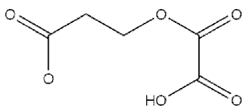
3-[(carboxycarbonyl)oxy]propanoic acid (Compound 37)
