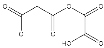
3-[(carboxycarbonyl)oxy]-3-oxopropanoic acid (Compound 36)
