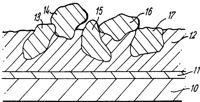
Fig. 1 PRIOR ART
