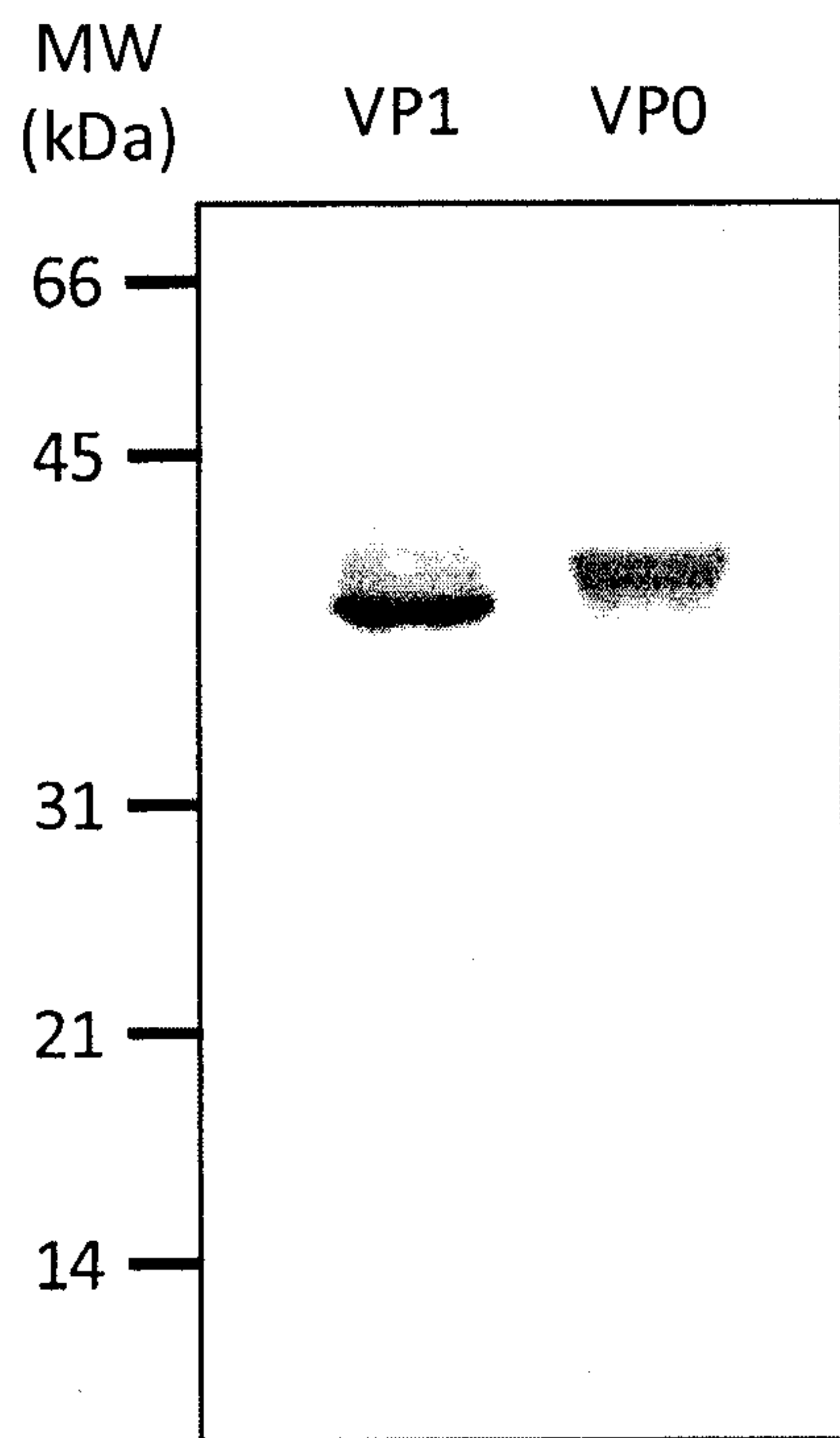
Figure 5. VP1 and VP0 are in the retentate after ultrafiltration over a 100kDa molecular weight cut off (MWCO) membrane.
