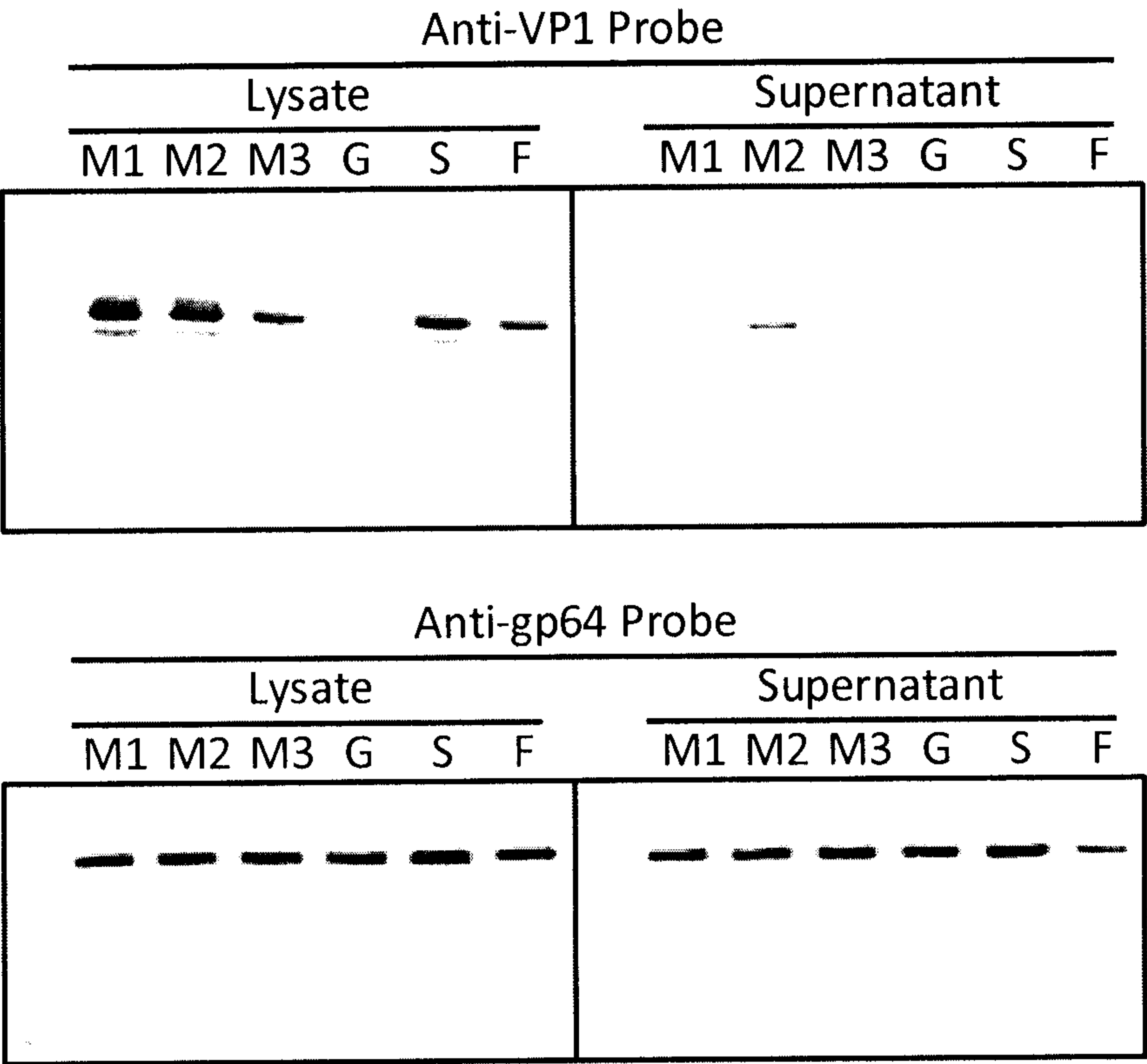
Figure 15. Comparison of expression of different recombinant baculovirus designs for expression of HEV71 VLP's.
