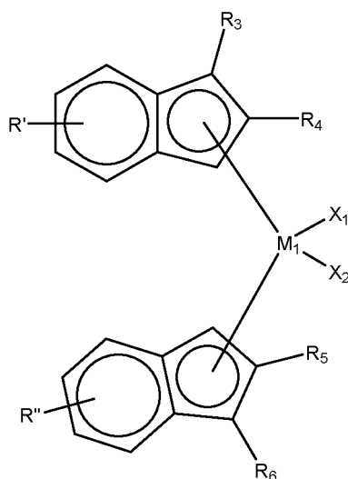
[Chemical Formula 1-4]
