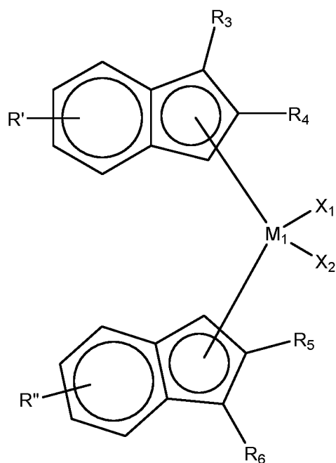
[Chemical Formula 1-4]
