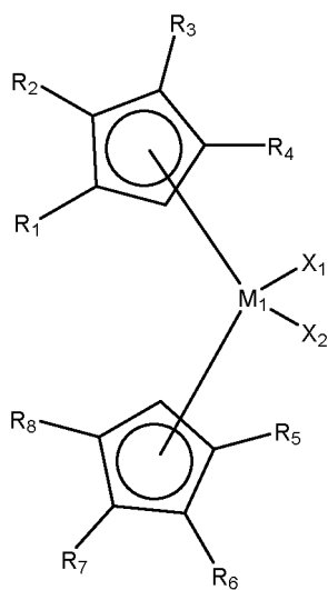
[Chemical Formula 1-2]
