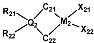
[Chemical Formula 2]
