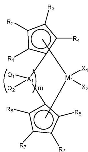
[Chemical Formula 1]
