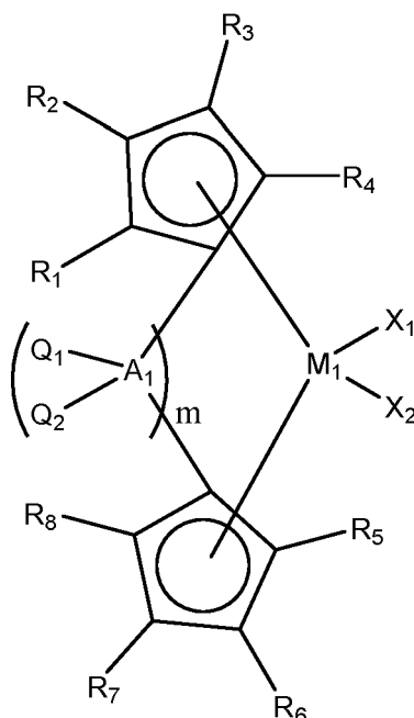
[Chemical Formula 1]
