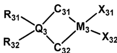
[Chemical Formula 3]
