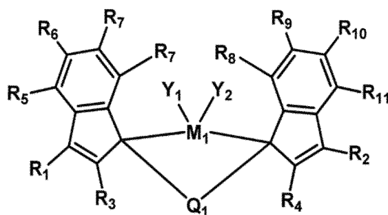
[Chemical Formula 1]
