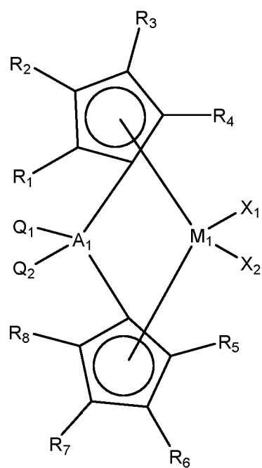
[Chemical Formula 1-3]
