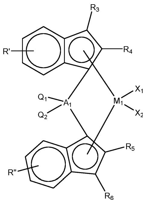
[Chemical Formula 1-4]
