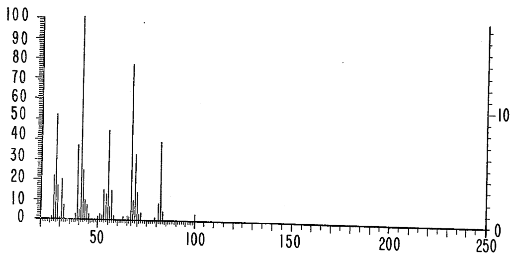
MASS SPECTRUM FOR EXAMPLE II.
