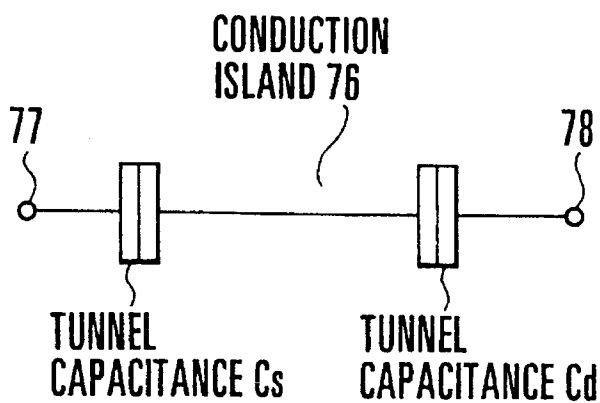
FIG. 32 PRIOR ART
