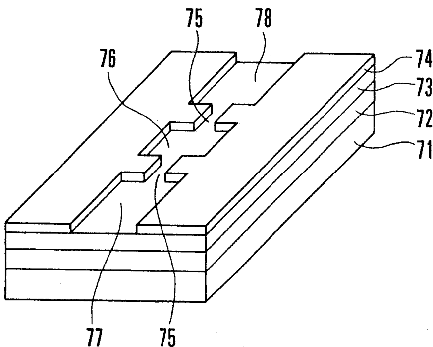
FIG. 31 PRIOR ART
