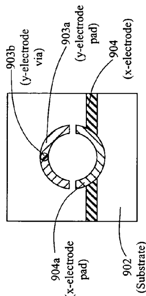
Figure 9C Top View - substrate and electrodes
