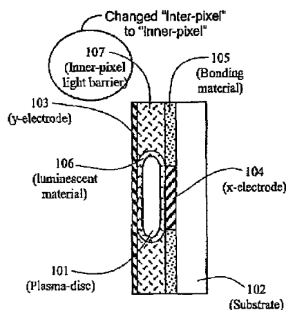
Section B-B View
