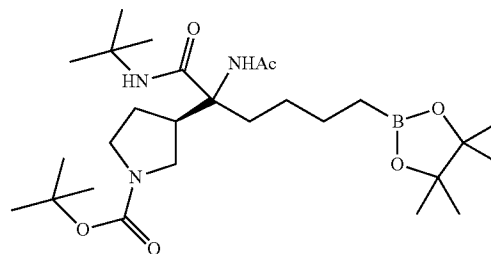
Step 4: ten-butyl (3R)-3-[1-acetamido-1-(tert-butylcarbamoyl)-5-(4,4,5,5-tetramethyl-1,3,2-dioxaborolan-2-yl)pentyl]pyrrolidine-1-carboxylate
