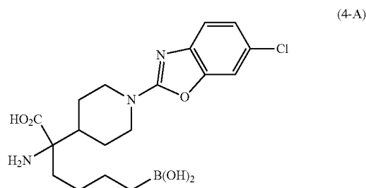
Step 7: 2-amino-6-borono-2-(1-(6-chlorobenzo[d]oxazol-2-yl)piperidin-4-yl)hexanoic acid
