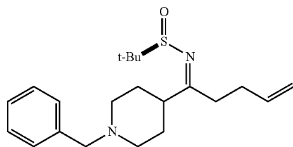
Step 3: (R,Z)—N-(1-(1-benzylpiperidin-4-yl)pent-4-enylidene)-2-methylpropane-2-sulfonamide
