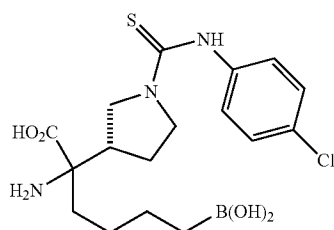
Step 6: 2-amino-6-borono-2-((S)-1-(4-chlorophenylcarbamothioyl)pyrrolidin-3-yl)hexanoic acid dihydrochloride
