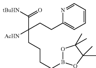
Step 6: 2-acetamido-N-tert-butyl-2-(2-(pyridin-2-yl)ethyl)-6-(4,4,5,5-tetramethyl-1,3,2-dioxaborolan-2-yl)hexanamide
