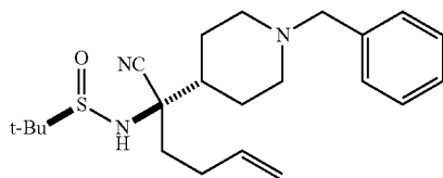
Step 4: (R)—N—((R)-1-(1-benzylpiperidin-4-yl)-1-cyanopent-4-enyl)-2-methylpropane-2-sulfonamide
