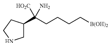
Step 5: (R)-2-amino-6-borono-2-((R)-pyrrolidin-3-yl)hexanoic acid
