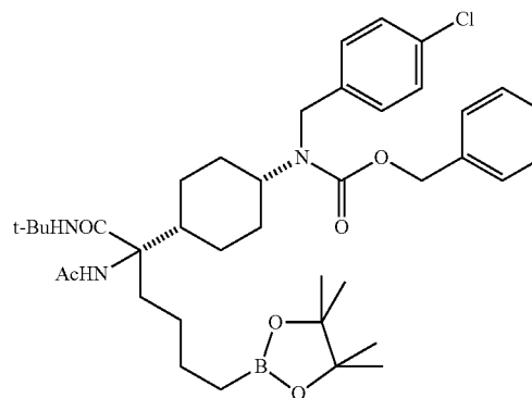
Step 5: benzyl (1R,4s)-4-((S)-2-acetamido-1-(tert-butylamino)-1-oxo-6-(4,4,5,5-tetramethyl-1,3,2-dioxaborolan-2-yl)hexan-2-yl)cyclohexyl(4-chlorobenzyl)carbamate
