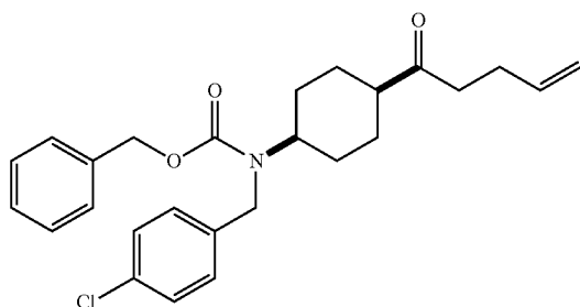
Step 3: 1-benzyl 4-chlorobenzyl(cis-4-pent-4-enoyl)cyclohexylcarbamate
