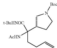
Step 3: 2-Acetamido-N-tert-butyl-2-[(3R)-1-tert-butylcarboxylpyrrolidin-3-yl]hex-5-enamide
