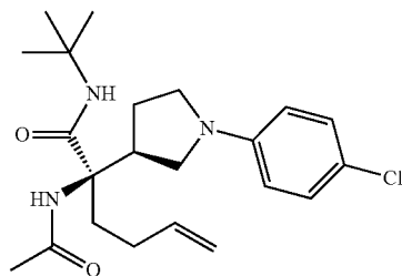
Step 3: (2S,3'S)-2-Acetylamino-2-[1-(4-chlorophenyl)-pyrrolidin-3-yl]-hex-5-enoic acid, tert-butylamide
