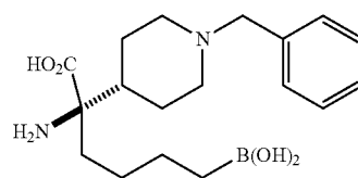
Step 6: (R)-2-amino-2-(1-benzylpiperidin-4-yl)-6-boronohexanoic acid
