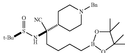
Step 5: (R)—N—((R)-1-(1-benzylpiperidin-4-yl)-1-cyano-5-(4,4,5,5-tetramethyl-1,3,2-dioxaborolan-2-yl)pentyl)-2-methylpropane-2-sulfonamide
