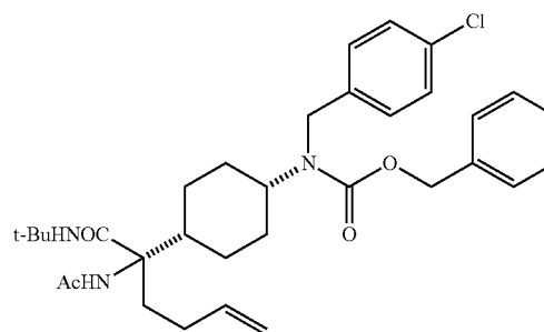
Step 4: benzyl (1R,4s)-4-((S)-2-acetamido-1-(tert-butylamino)-1-oxohex-5-en-2-yl)cyclohexyl(4-chlorobenzyl)carbamate
