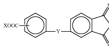
Structural Formula (3)
