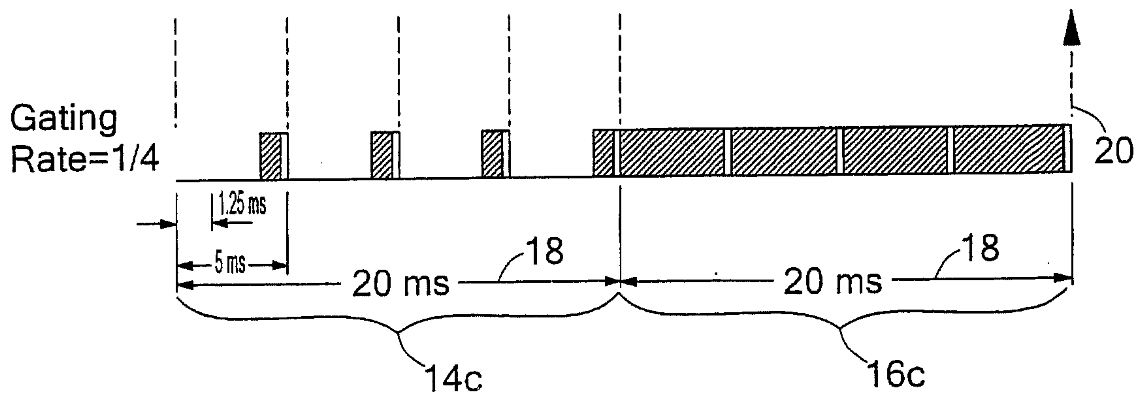
FIG. 1C Prior Art
