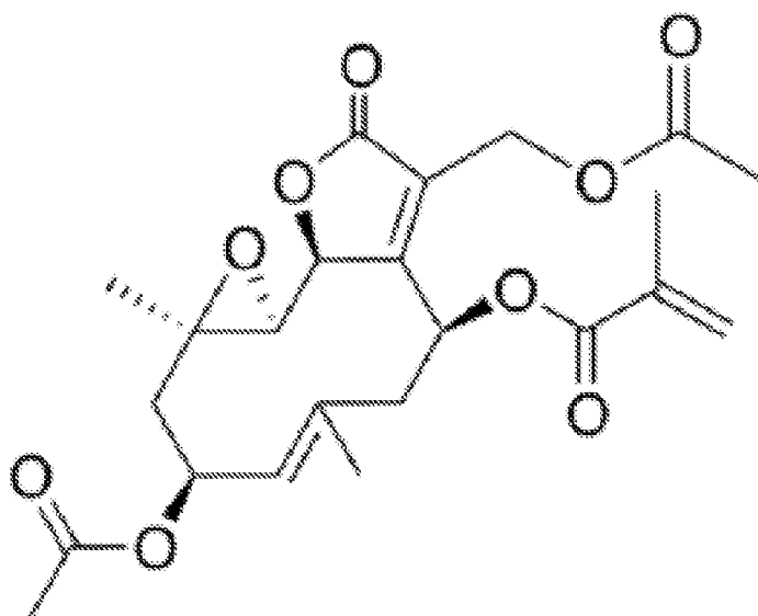
Glaucolide E LD_{50} = 1.12 \mu M
