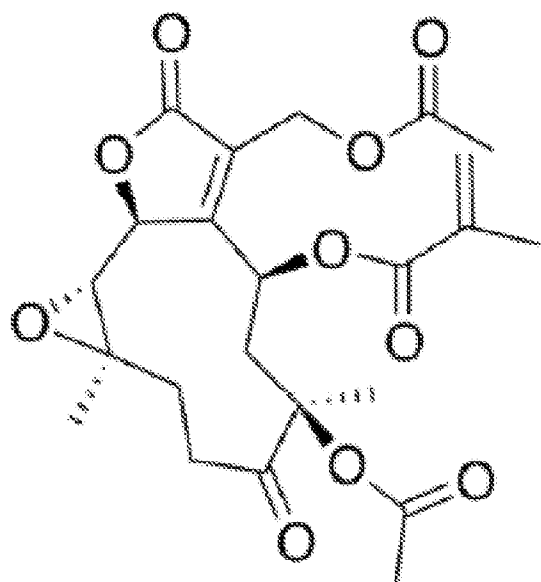
Glaucolide A LD_{50} = 1.82 \mu M
