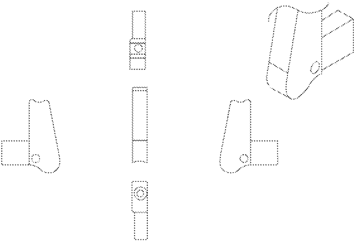
Rotatable Saddle 182
