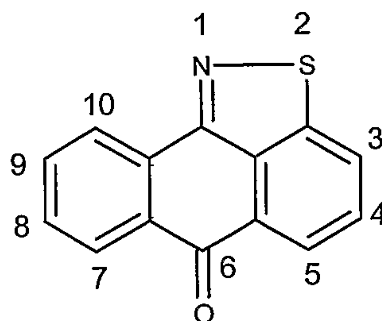
Anthra[9,1- cd ]isothiazol-6-one (IIIE)
