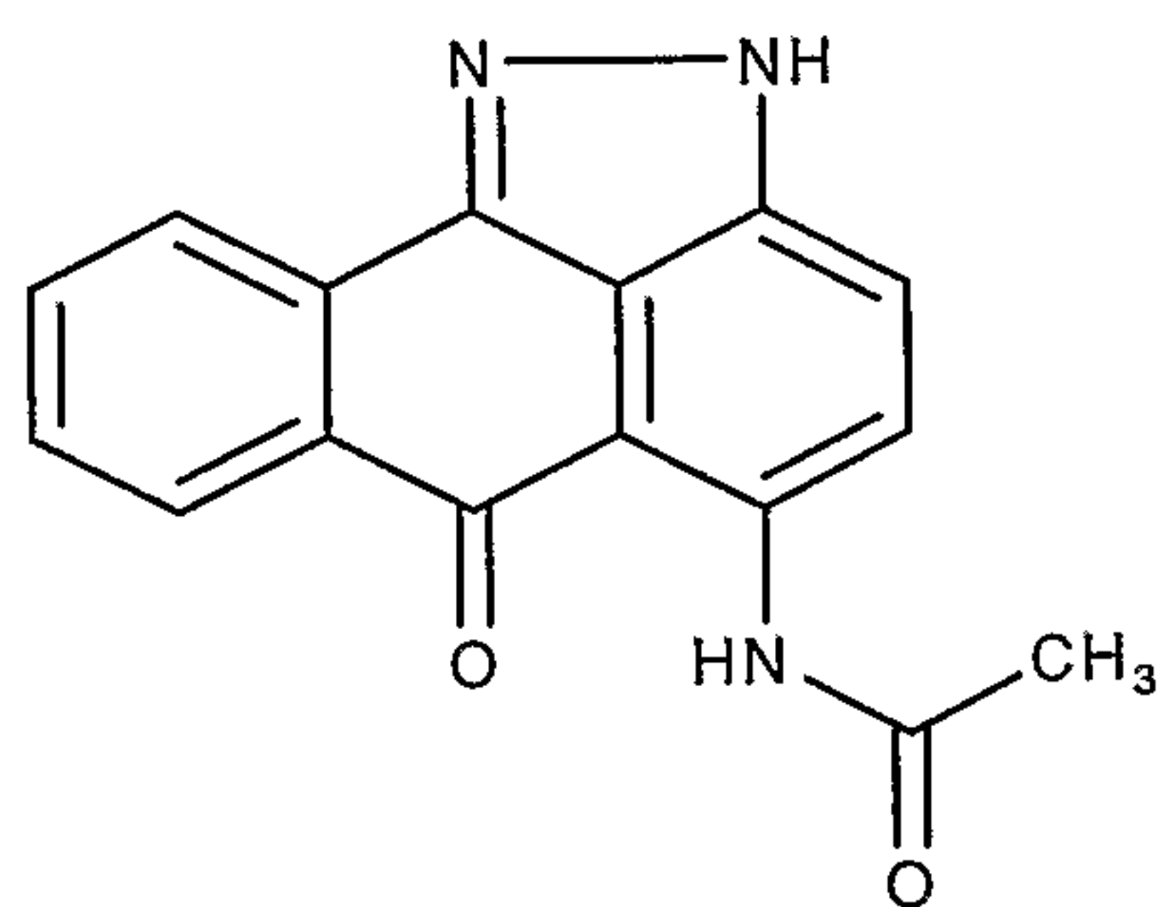
N-(6-Oxo-2,6-dihydro- dibenzo[ cd,g ]indazol-5-yl)- acetamide ;
