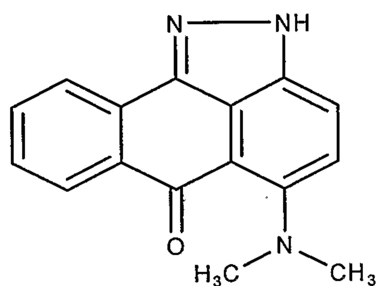
5-Dimethylamino-2 H - dibenzo[ cd,g ]indazol-6-one;
