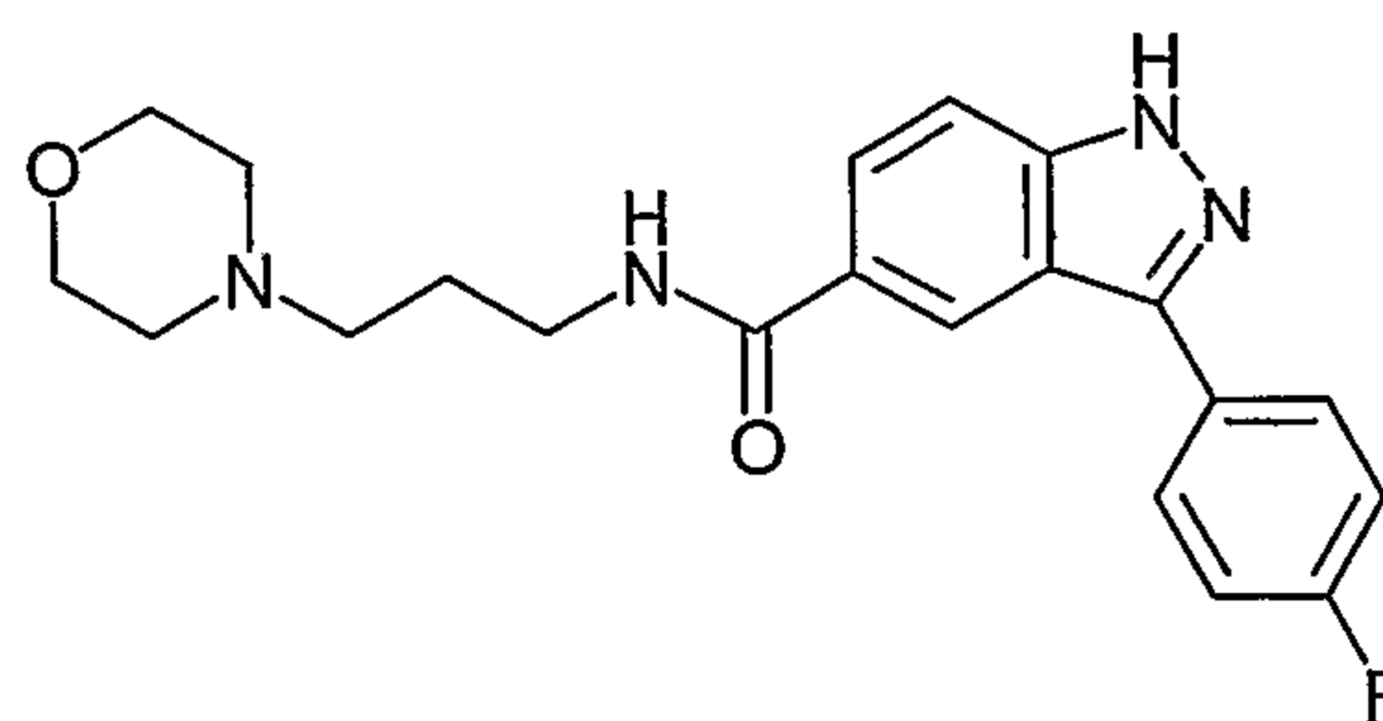
3-(4-Fluoro-phenyl)-1 H -indazole-5-carboxylic acid (3-morpholin-4-yl-propyl)-amide ;
