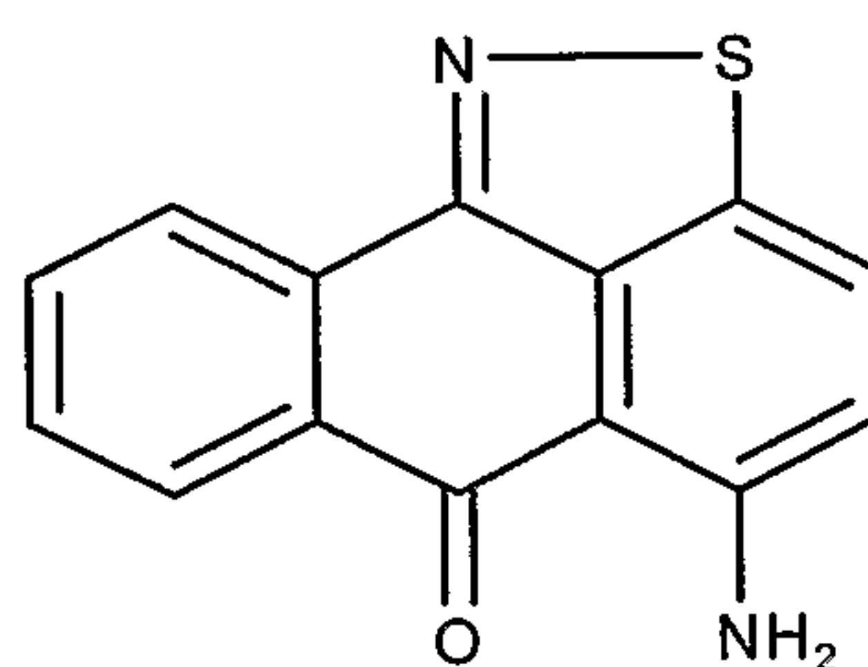
5-Amino-anthra[9,1- cd ]isothiazol-6-one ;
