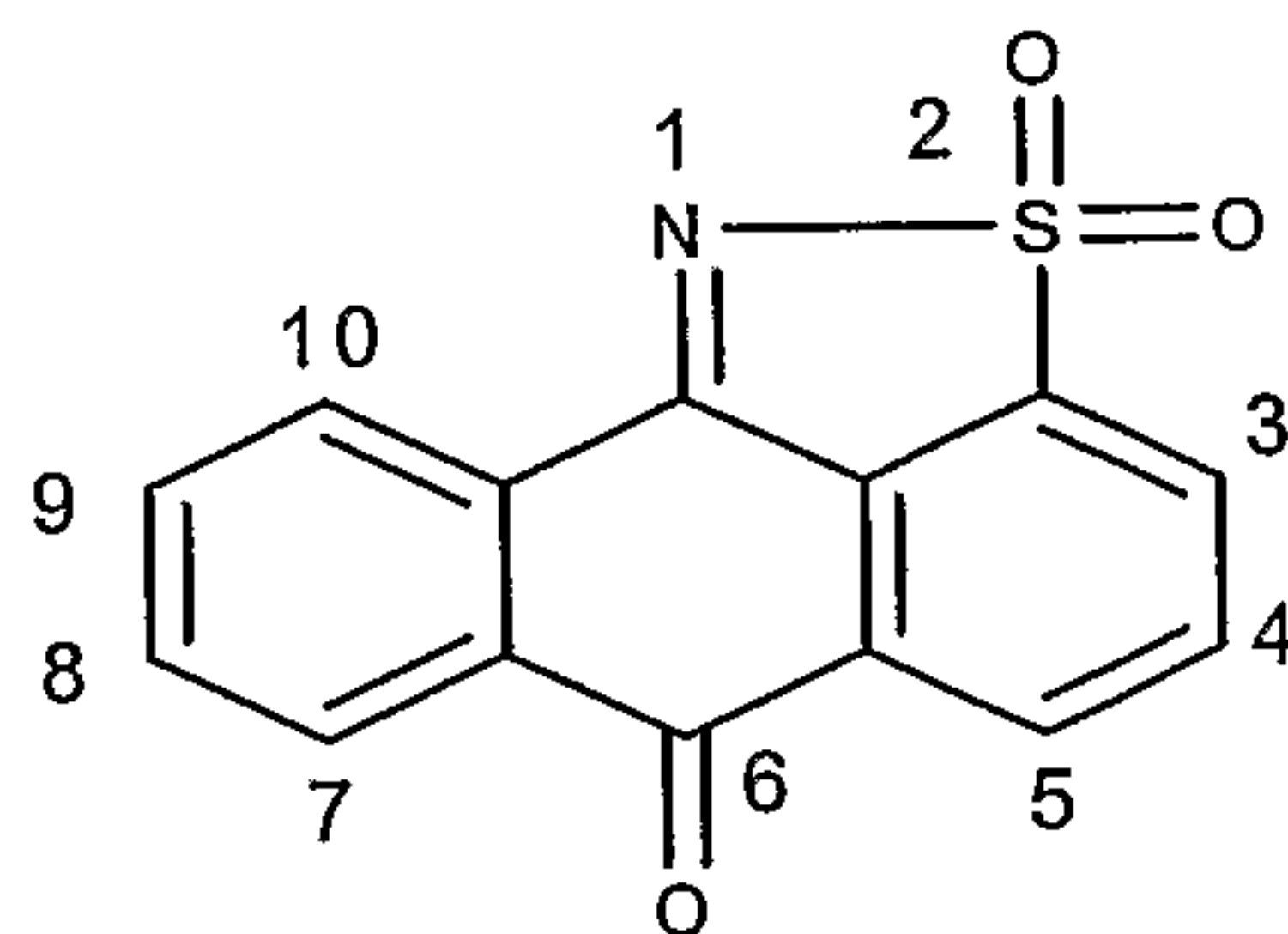
2,2-Dioxo-2H-21 6 -anthra [9,1-cd]isothiazol-6-one (IIID)
