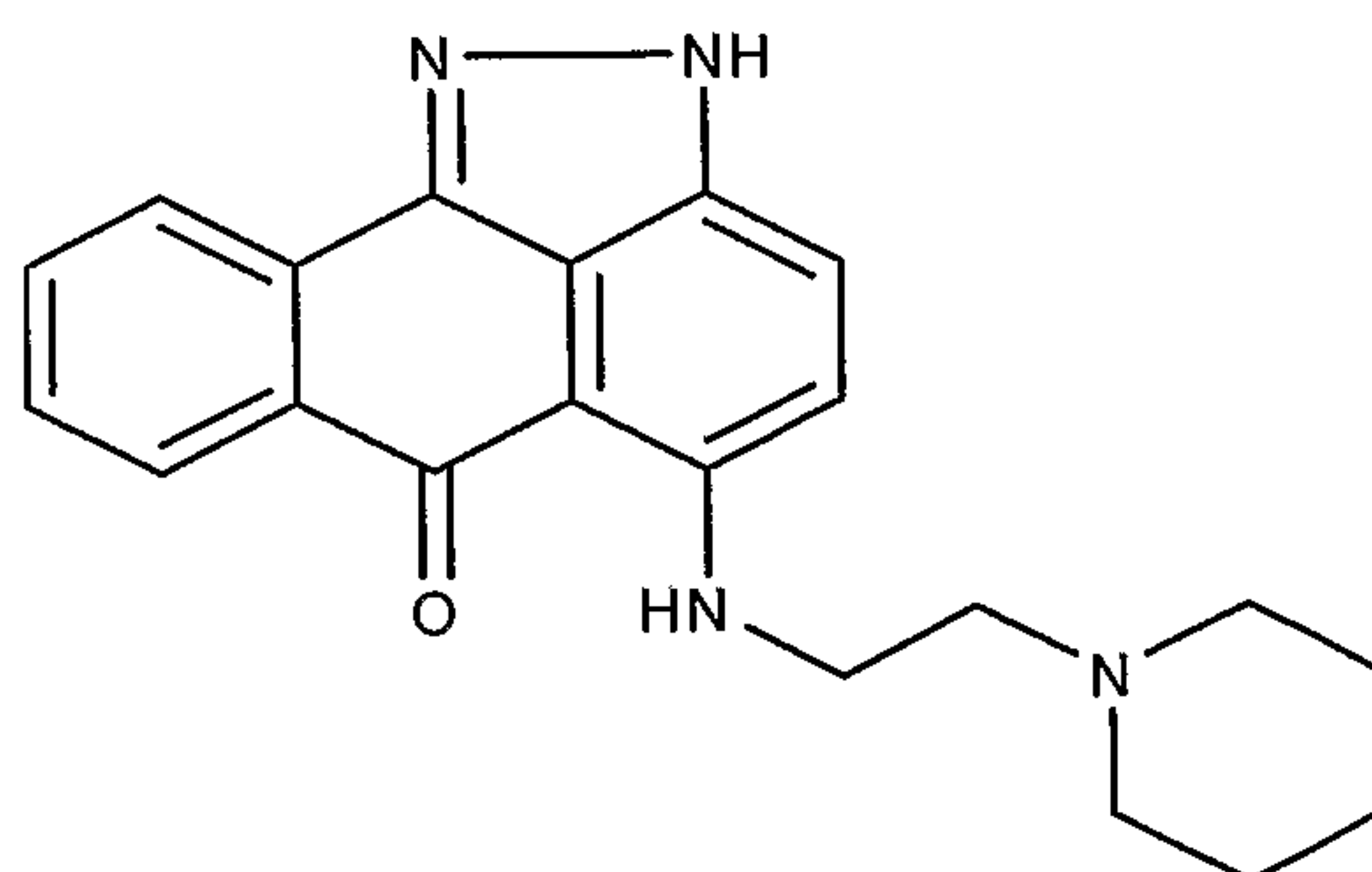
5-(2-Piperidin-1-yl-ethylamino)-2 H - dibenzo[ cd,g ]indazol-6-one ;
