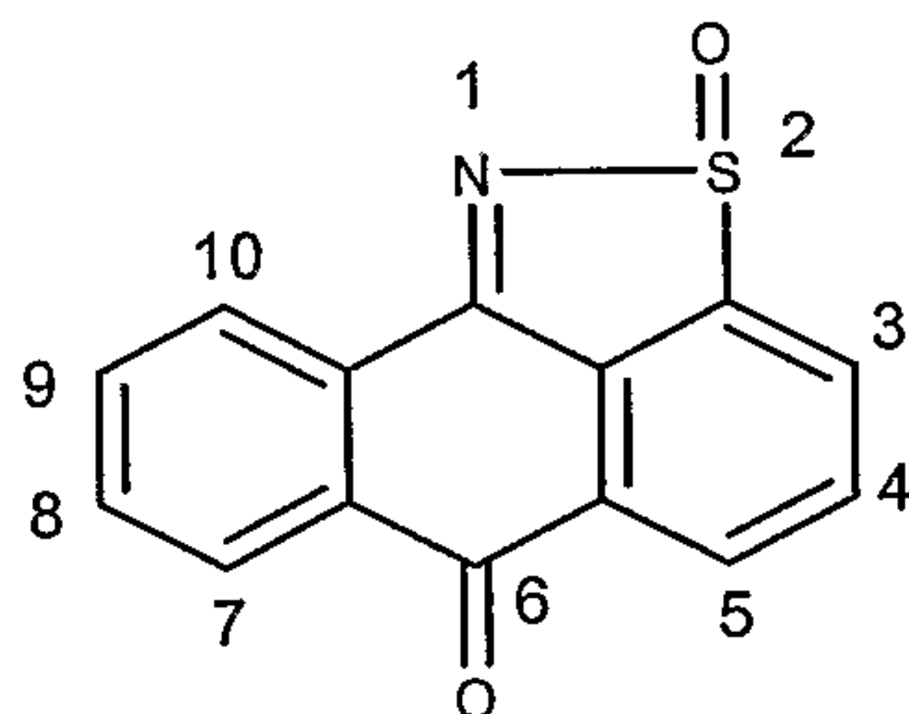
2-Oxo-2H-21 4 -anthra[9,1-cd] isothiazol-6-one (IIIB)
