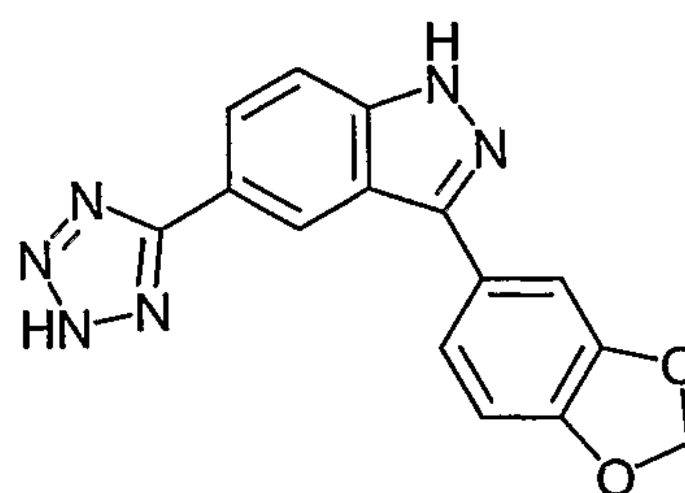
3-Benzo[1,3]dioxol-5-yl-5-(2 H -tetrazol- 5-yl)-1 H -indazole ;
