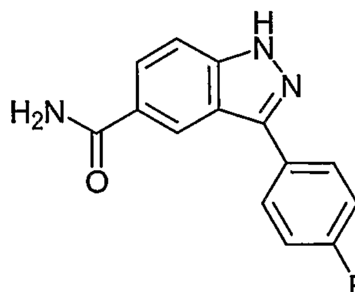
3-(4-Fluoro-phenyl)-1H-indazole-5-carboxylic acid amide ;
