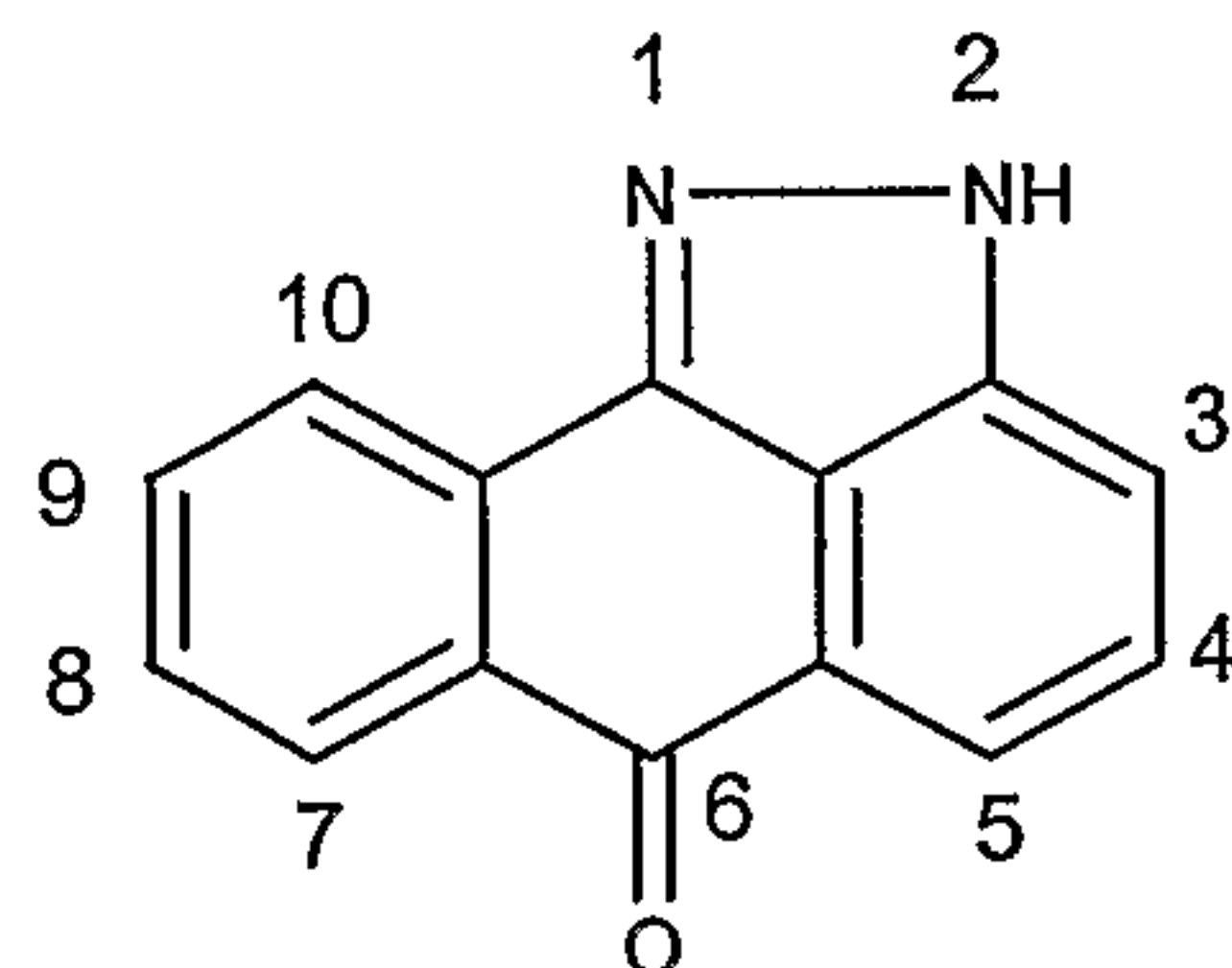
2H-Dibenzo[ cd,g ]indazol-6-one (IIIF)
