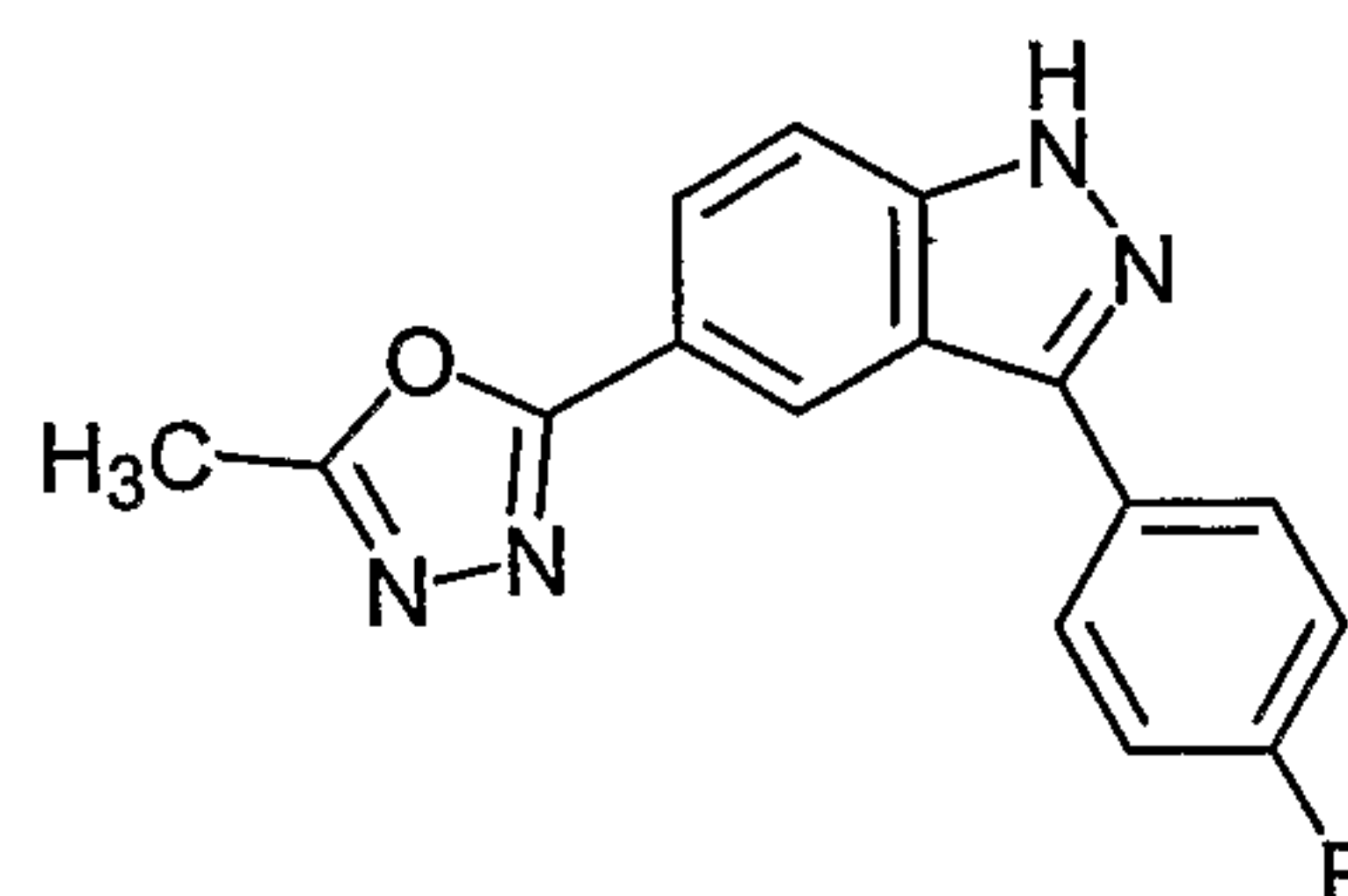
3-(4-Fluoro-phenyl)-5-(5- methyl-[1,3,4]oxadiazol-2-yl)- 1 H -indazole ;
