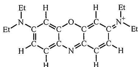
basic blue 3
