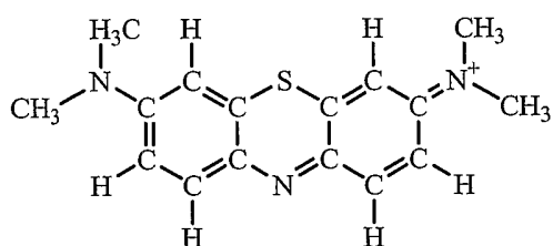
methylene blue
