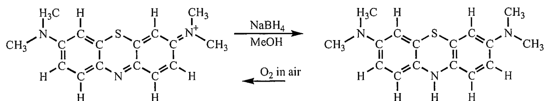
methylene blue
