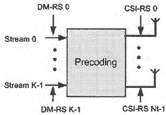
Figure 4 - UE-specific precoded DM-RS
