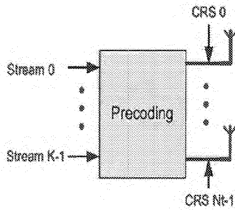
Figure 5 - Non-precoded cell-specific RS
