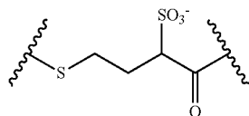
4-thio-2-hydroxysulfonyl-butyrate (2-Sulfo-SPDB),
