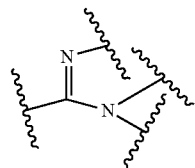
acetimidamide
