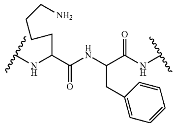
lysine-phenylalanine (lys-phe)
