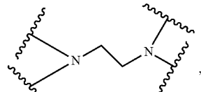
acetylaceto-hydrazide
