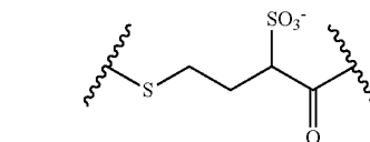
4-thio-2-hydroxysulfonyl-butyrate (2-Sulfo-SPDB),
