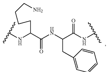
lysine-phenylalanine (lys-phe)
