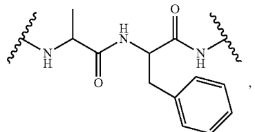
alanine-phenylalanine (ala-phe)
