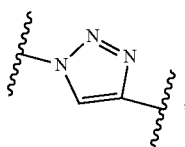
triazole
