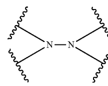
hydrazine
