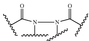
acetylaceto-hydrazide
