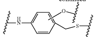
amino-oxylbenzylthio
