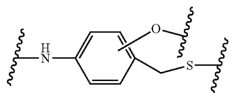
amino-oxybenzylthio
