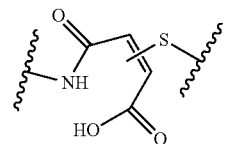
thio-amino-oxobutenoic acid,
