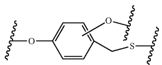
dioxylbenzylthio
