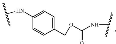
p-aminobenzoyloxycarbonyl (PAB)
