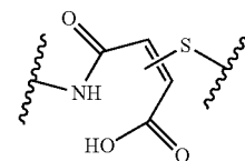
thio-amino-oxobutanoic acid,
