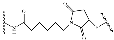
6-maleimidocaproyl (MC)
