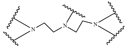
aminoethyl-aminoethyl-amine
