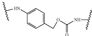
p-aminobenzyloxycarbonyl (PAB)
