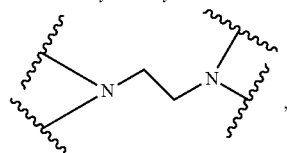
ami-noethyl-amine
