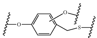
dioxybenzylthio
