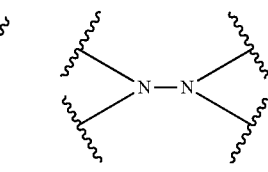
hydrazine
