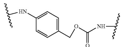
p-aminobenzoyloxycarbonyl (PAB)
