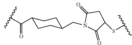
4-(N-maleimidomethyl)cyclo-hexane-1-carboxylate (MCC),
