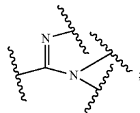
acetimidamide
