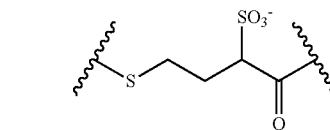
4-thio-2-hydroxysulfonyl-butyrate (2-Sulfo-SPDB),
