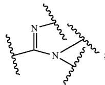
acetimidamide
