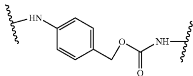
p-aminobenzyloxycarbonyl (PAB)
