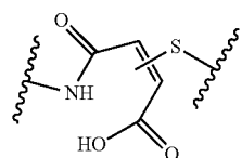
thio-amino-oxobutanoic acid,
