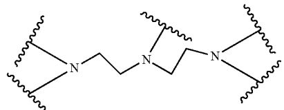
aminoethyl-aminoethyl-amine
