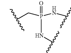
N,N'-dimethylphosphondiamide,
