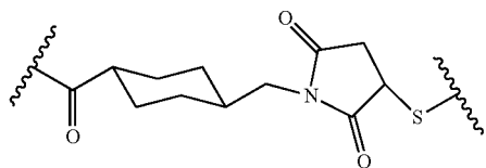
4-(N-maleimidomethyl)cyclo-hexane-1-carboxylate (MCC),
