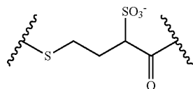
4-thio-hydroxysulfonyl-butyrate (2-Sulfo-SPDB),
