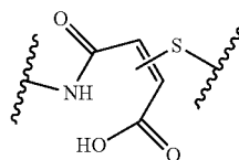
thio-amino-oxobutanoic acid,
