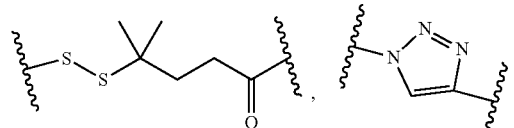
4-methyl-4-dithio-pentanoic (MPDP)
