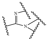
acetimidamide
