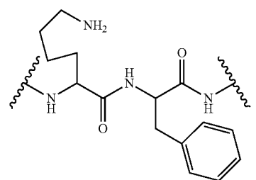
lysine-phenylalanine (lys-phe)
