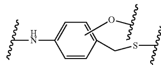
amino-oxybenzylthio
