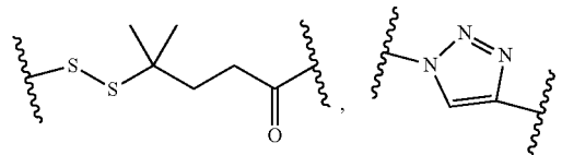
4-methyl-4-dithio-pentanoic (MPDP)
