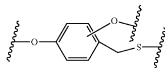
dioxybenzylthio
