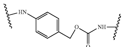
p-aminobenzoyloxycarbonyl (PAB)
