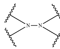
hydrazine
