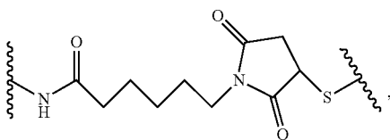
6-maleimidocaproyl (MC)
