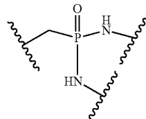
N,N'-dimethylphosphondiamide,
