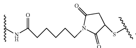
6-maleimidocaproyl (MC)
