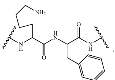
lysine-phenylalanine (lys-phe)
