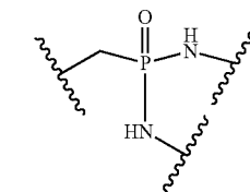
N,N'-dimethylphosphondiamide,
