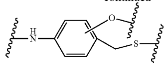
amino-oxybenzylthio
