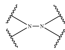
hydrazine
