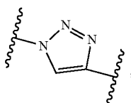
triazole
