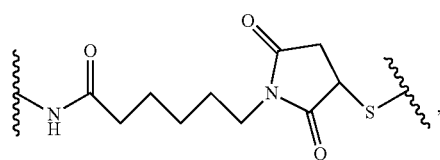
6-maleimidocaproyl (MC)
