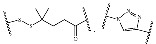
4-methyl-4-dithio-pentanoic (MPDP)
