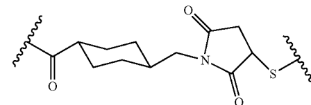
4-(N-maleimidomethyl)cyclo-hexane-1-carboxylate (MCC),
