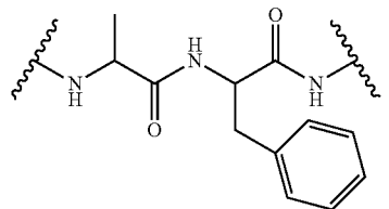
alanine-phenylalanine (ala-phe)
