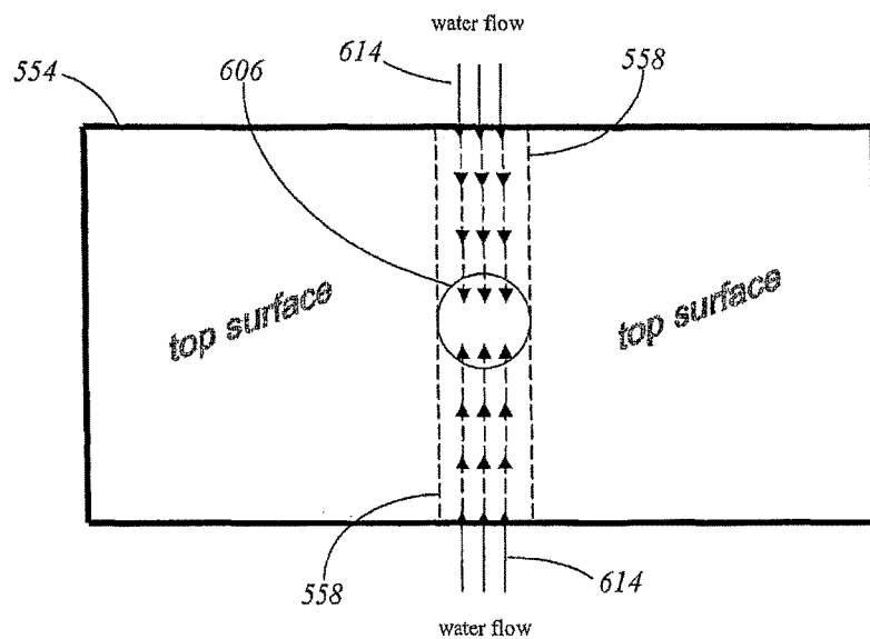
FIG. 16B top view
