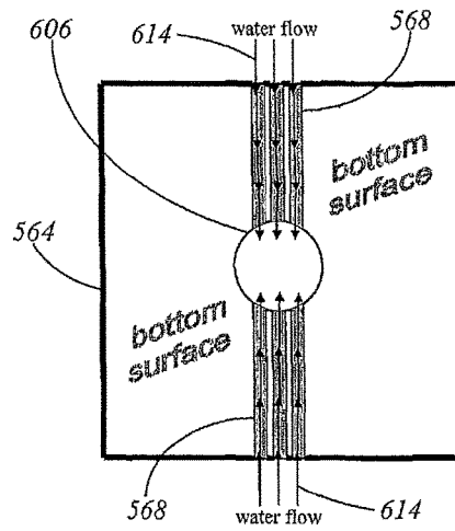
FIG. 17B bottom view
