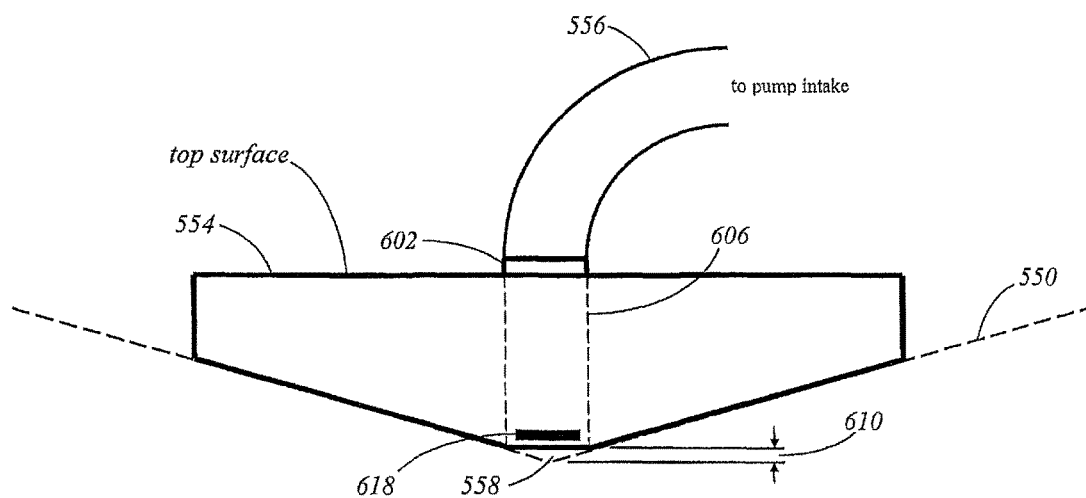
FIG. 16A side view
