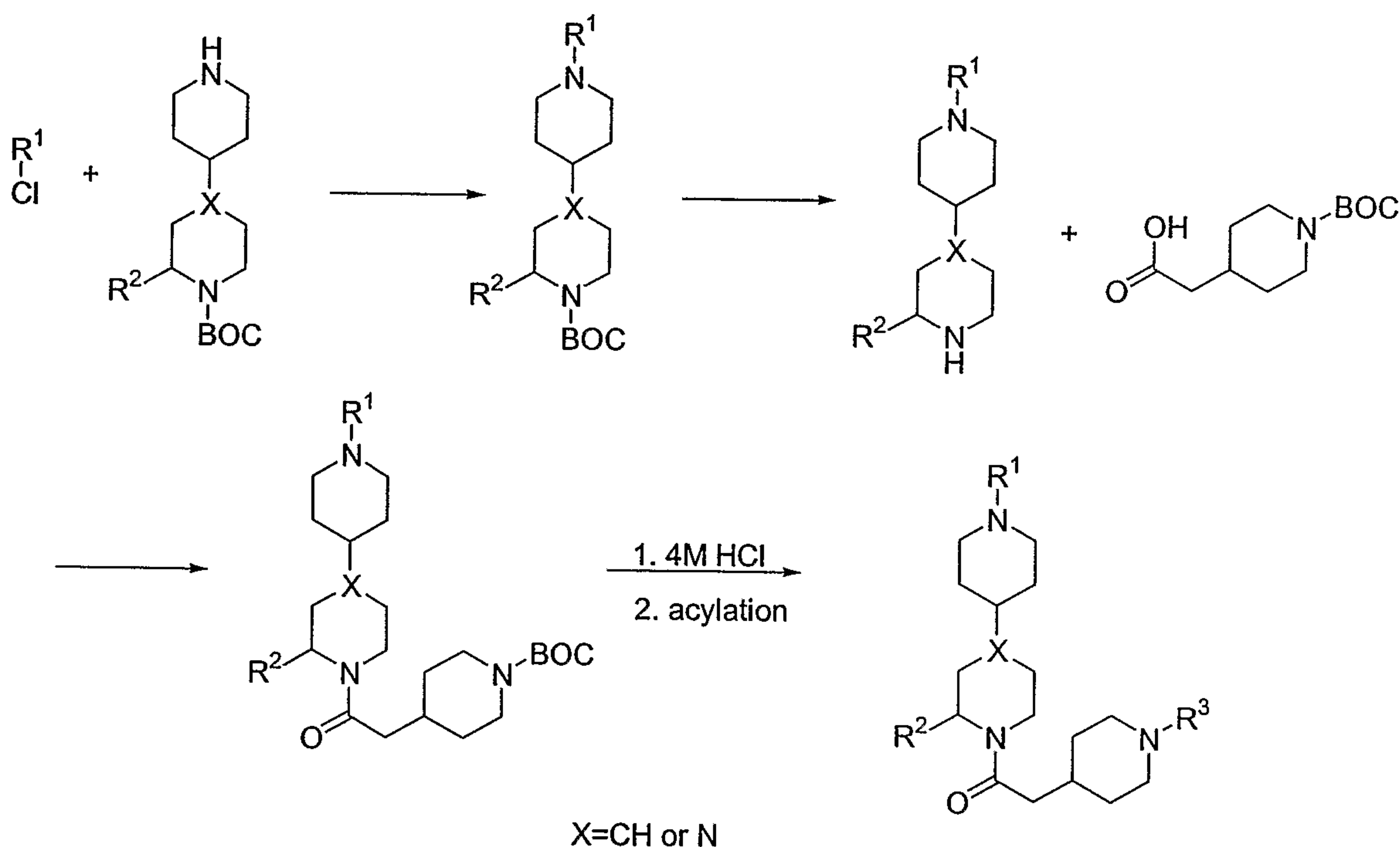
Scheme 1
