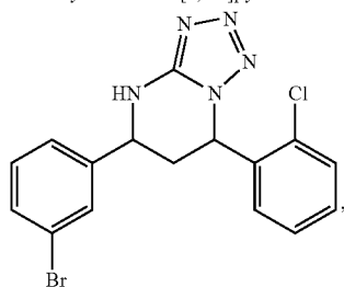
(+/-)-(cis)-5-(3-bromophenyl)-7-(2-chlorophenyl)-4,5,6,7-tetrahydrotriazolo[1,5-a]pyrimidine
