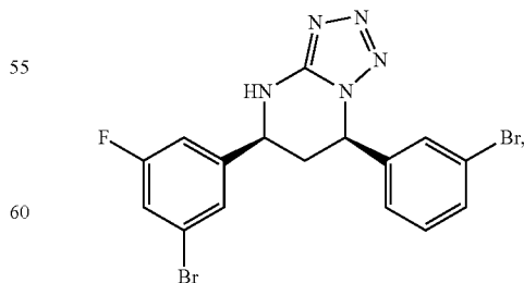
(5S,7R)-5-(3-bromo-5-fluorophenyl)-7-(3-bromophenyl)-4,5,6,7-tetrahydrotriazolo[1,5-a]pyrimidine 1
