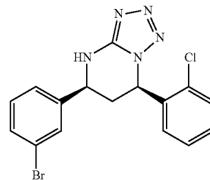
(5S,7R)-5-(3-bromophenyl)-7-(2-chlorophenyl)-4,5,6,7-tetrahydro-1,5-a-pyridine 1
