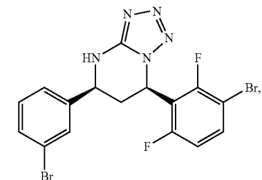
(5S,7R)-7-(3-bromo-2,6-difluorophenyl)-5-(3-bromophenyl)-4,5,6,7-tetrahydro-1H-tetrazolo[1,5-a]pyrimidine 1
