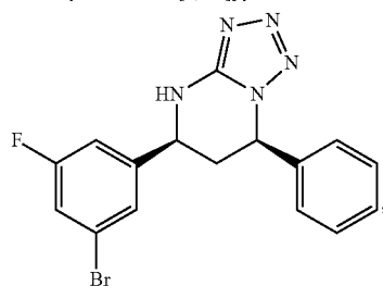
((5S,7R))-5-(3-bromo-5-fluorophenyl)-7-phenyl-4,5,6,7-tetrahydrotriazolo[1,5-a]pyrimidine 1
