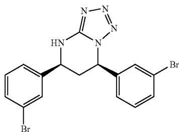
((5S,7R))-5,7-bis(3-bromophenyl)-4,5,6,7- tetrahydro-tetrazolo[1,5-a]pyrimidine
