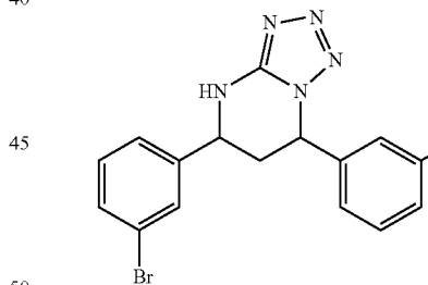
(+/-)-(cis)-5-(3-bromophenyl)-7-(3-chlorophenyl)-4,5,6,7-tetrahydrotriazolo[1,5-a]pyrimidine
