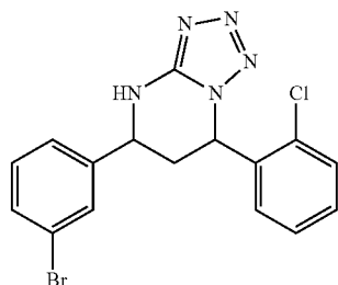
(+/-)-(cis)-5-(3-bromophenyl)-7-(2-chlorophenyl)-4,5,6,7-tetrahydro-1,5-a-pyridine
