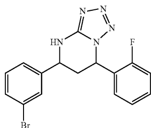
(+/-)-(cis)-5-(3-bromophenyl)-7-(2-fluorophenyl)-4,5,6,7-tetrahydro-1,5-a-pyridine
