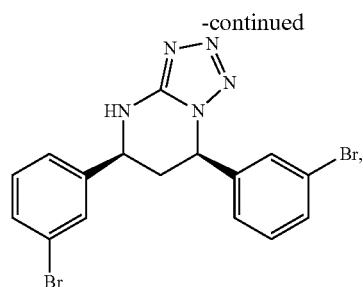
(5S,7R)-5,7-bis(3-bromophenyl)-4,5,6,7-tetrahydro-1H-tetrazolo[1,5-a]pyrimidine
