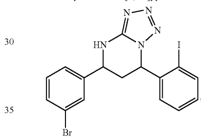
(+/-)-(cis)-5-(3-bromophenyl)-7-(2-iodophenyl)-4,5,6,7-tetrahydrotriazolo[1,5-a]pyrimidine
