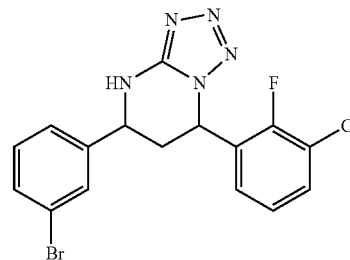
(+/-)-(cis)-5-(3-bromophenyl)-7-(3-chloro-2-fluorophenyl)- 4,5,6,7-tetrahydro-tetrazolo[1,5-a]pyrimidine
