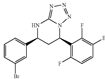
((5S,7R))-7-(3-bromo-2,6-difluorophenyl)-5-(3-bromophenyl)- 4,5,6,7-tetrahydro-tetrazolo[1,5-a]pyrimidine 1
