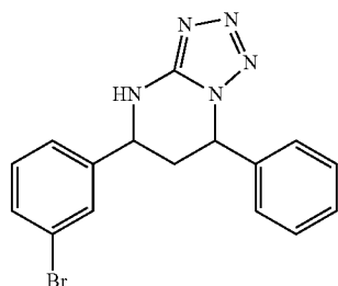
(+/-)-(cis)-5-(3-bromophenyl)-7-phenyl-4,5,6,7-tetrahydro-1,5-a-pyridine
