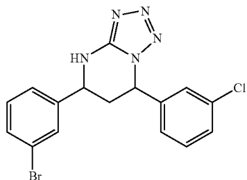
(+/-)-(cis)-5-(3-bromophenyl)-7-(3-chlorophenyl)- 4,5,6,7-tetrahydro-tetrazolo[1,5-a]pyrimidine
