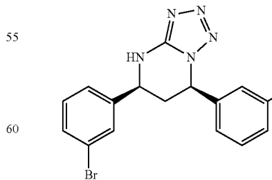
((5S,7R))-5-(3-bromophenyl)-7-(3-chlorophenyl)-4,5,6,7-tetrahydrotriazolo[1,5-a]pyrimidine 1
