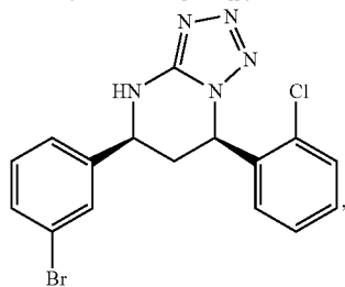
((5S,7R))-5-(3-bromophenyl)-7-(2-chlorophenyl)-4,5,6,7-tetrahydrotriazolo[1,5-a]pyrimidine 1
