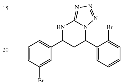
(+/-)-(cis)-7-(2-bromophenyl)-5-(3-bromophenyl)-4,5,6,7-tetrahydrotriazolo[1,5-a]pyrimidine
