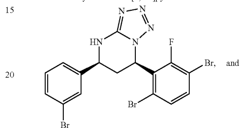
(5S,7R)-5-(3-bromophenyl)-7-(3,6-dibromo-2-fluorophenyl)-4,5,6,7-tetrahydro-1H-tetrazolo[1,5-a]pyrimidine 1
