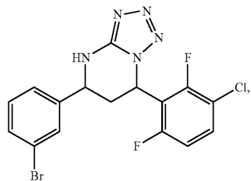
(+/-)-(cis)-5-(3-bromophenyl)-7-(3-chloro-2,6-difluorophenyl)-4,5,6,7-tetrahydro-1H-tetrazolo[1,5-a]pyrimidine
