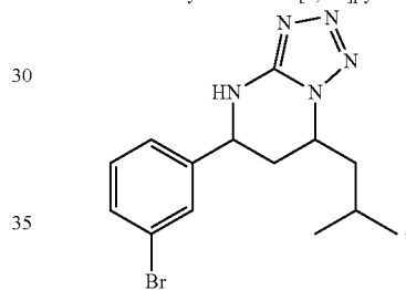
(+/-)-(cis)-5-(3-bromophenyl)-7-isobutyl-4,5,6,7-tetrahydro-1H-tetrazolo[1,5-a]pyrimidine
