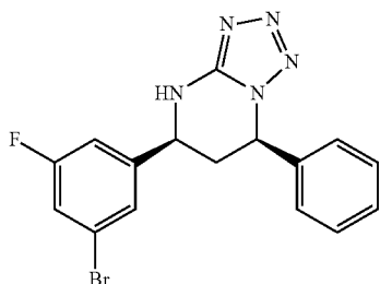
(5S,7R)-5-(3-bromo-5-fluorophenyl)-7-phenyl-4,5,6,7-tetrahydro-1,5-a-pyridine 1
