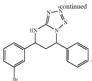
(+/-)-(cis)-5-(3-bromophenyl)-7-phenyl-4,5,6,7-tetrahydrotriazolo[1,5-a]pyrimidine
