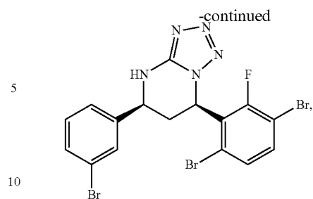
(5S,7R)-7-(3-bromophenyl)-7-(3,6-dibromo-2-fluorophenyl)-4,5,6,7-tetrahydro-1H-tetrazolo[1,5-a]pyrimidine 1
