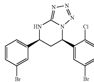
((5S,7R))-7-(5-bromo-2-chlorophenyl)-5-(3-bromophenyl)- 4,5,6,7-tetrahydro-tetrazolo[1,5-a]pyrimidine 1
