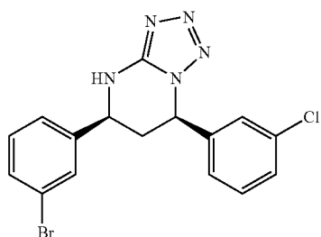
((5S,7R))-5-(3-bromophenyl)-7-(3-chlorophenyl)- 4,5,6,7-tetrahydro-tetrazolo[1,5-a]pyrimidine 1
