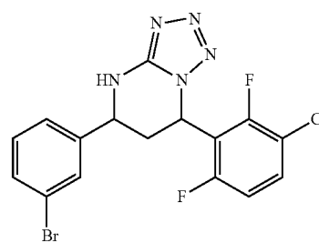
(+/-)-(cis)-5-(3-bromophenyl)-7-(3-chloro-2,6-difluorophenyl)- 4,5,6,7-tetrahydro-tetrazolo[1,5-a]pyrimidine
