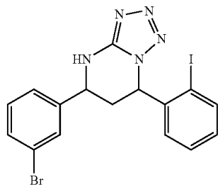
(+/-)-(cis)-5-(3-bromophenyl)-7-(2-iodophenyl)- 4,5,6,7-tetrahydro-tetrazolo[1,5-a]pyrimidine
