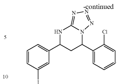
(+/-)-(cis)-7-(2-chlorophenyl)-5-(3-iodophenyl)-4,5,6,7-tetrahydrotriazolo[1,5-a]pyrimidine
