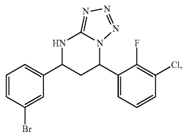
(+/-)-(cis)-5-(3-bromophenyl)-7-(3-chloro-2-fluorophenyl)-4,5,6,7-tetrahydro-1H-tetrazolo[1,5-a]pyrimidine
