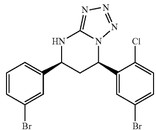
(5S,7R)-7-(5-bromo-2-chlorophenyl)-5-(3-bromophenyl)-4,5,6,7-tetrahydro-1H-tetrazolo[1,5-a]pyrimidine 1
