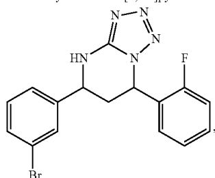
(+/-)-(cis)-5-(3-bromophenyl)-7-(2-fluorophenyl)-4,5,6,7-tetrahydrotriazolo[1,5-a]pyrimidine
