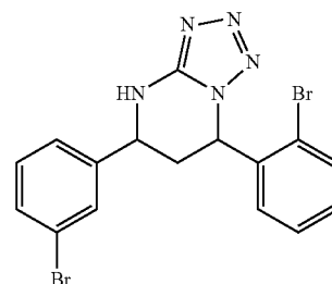
(+/-)-(cis)-7-(2-bromophenyl)-5-(3-bromophenyl)-4,5,6,7-tetrahydro-1,5-a-pyridine
