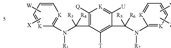
Formula Vc
