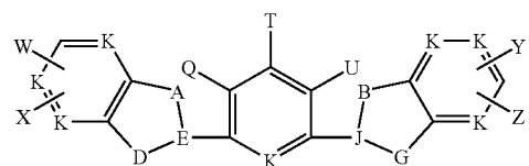
Formula VIb
