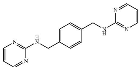
Formula XVI
