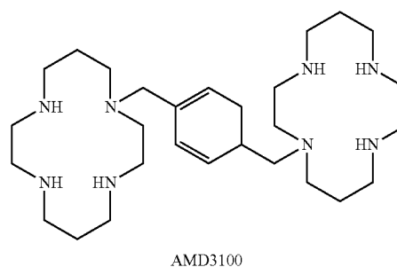
AMD3100
