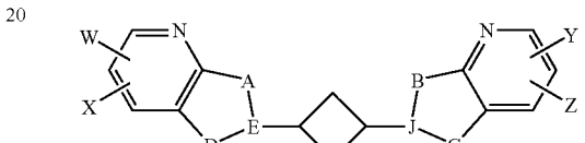
(X-1)
