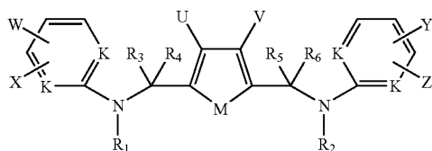
Formula VII
