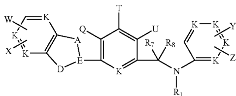
Formula VIb
