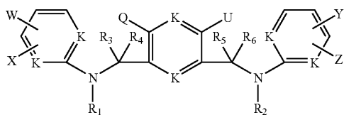
Formula Vb
