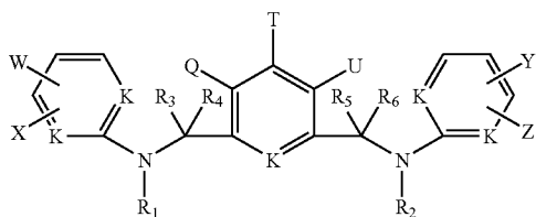
Formula Vb
