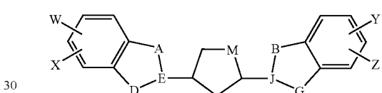
(X-2)
