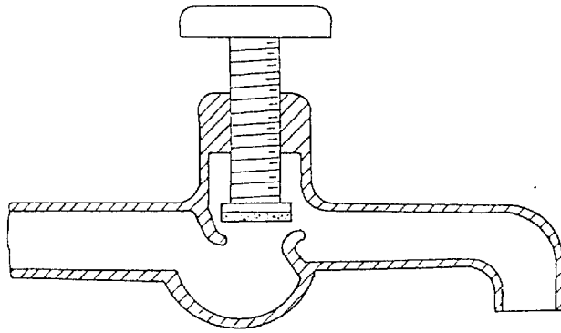
FIG. 1 PRIOR ART
