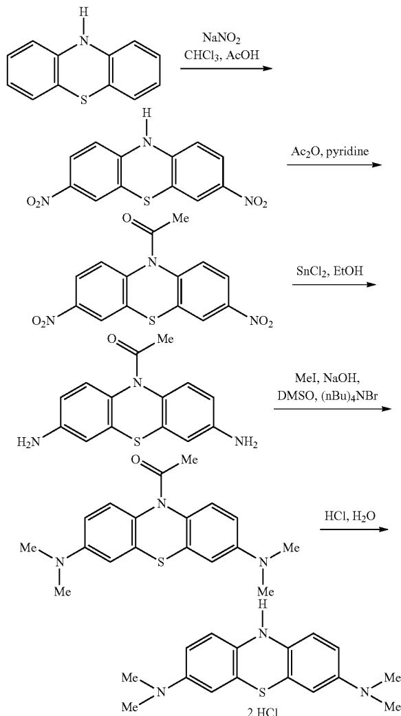
Scheme 1
