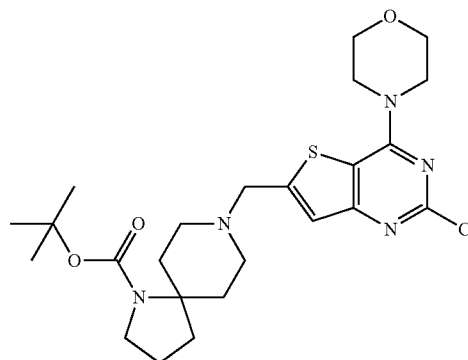
8-(2-Chloro-4-morpholin-4-yl-thieno[3,2-d]pyrimidin-6-ylmethyl)-1,8-diaza-spiro[4.5]decane-1-carboxylic acid tert-butyl ester
