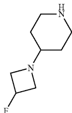
4-(3-Fluoroazetidin-1-yl)-piperidine
