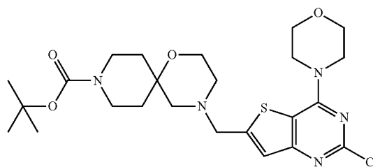
4-(2-Chloro-4-morpholin-4-yl-thieno[3,2-d]pyrimidin-6-ylmethyl)-1-oxa-4,9-diaza-spiro[5.5]undecane-9-carboxylic acid tert-butyl ester
