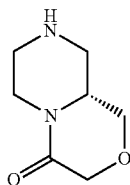
(R)-Hexahydro-pyrazino[2,1-c][1,4]oxazin-4-one
