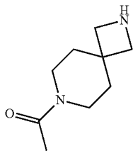
1-(2,7-Diaza-spiro[3.5]non-7-yl)-ethanone
