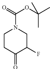
3-Fluoro-4-oxo-piperidine-1-carboxylic acid tert-butyl ester
