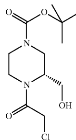
(R)-4-(2-Chloro-acetyl)-3-hydroxymethyl-piperazine-1-carboxylic acid tert-butyl ester
