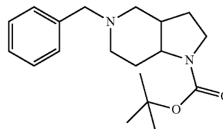
5-Benzyl-octahydro-pyrrolo[3,2-c]pyridine-1-carboxylic acid tert-butyl ester
