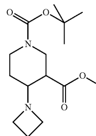
(±)-4-Azetidin-1-yl-piperidine-1,3-dicarboxylic acid 1-tert-butyl ester 3-methyl ester
