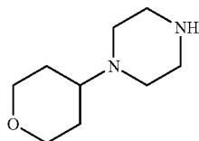
1-(Tetrahydro-pyran-4-yl)-piperazine
