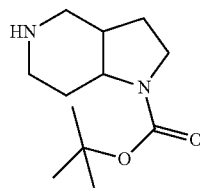
Octahydro-pyrrolo[3,2-c]pyridine-1-carboxylic acid tert-butyl ester
