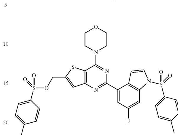
Toluene-4-sulfonic acid 2-[6-fluoro-1-(toluene-4-sulfonyl)-1H-indol-4-yl]-4-morpholin-4-yl-thieno[3,2-d]pyrimidin-6-ylmethyl ester
