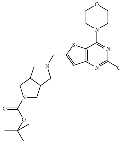
5-(2-Chloro-4-morpholin-4-yl-thieno[3,2-d]pyrimidin-6-ylmethyl)-hexahydro-pyrrolo[3,4-c]pyrrole-2-carboxylic acid tert-butyl ester
