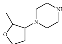
(±)-1-(2-Methyl-tetrahydro-furan-3-yl)-piperazine
