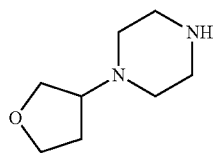
(±)-1-(Tetrahydro-furan-3-yl)-piperazine
