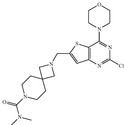
2-(2-Chloro-4-morpholin-4-yl-thieno[3,2-d]pyrimidin-6-ylmethyl)-2,7-diaza-spiro[3.5]nonane-7-carboxylic acid dimethylamide
