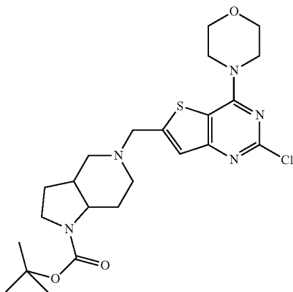
5-(2-Chloro-4-morpholin-4-yl-thieno[3,2-d]pyrimidin-6-ylmethyl)-octahydro-pyrrolo[3,2-c]pyridine-1-carboxylic acid tert-butyl ester
