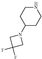
4-(3,3-Difluoroazetidin-1-yl)-piperidine
