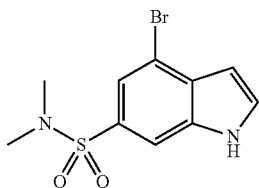
4-Bromo-1H-indole-6-sulfonic acid dimethylamide
