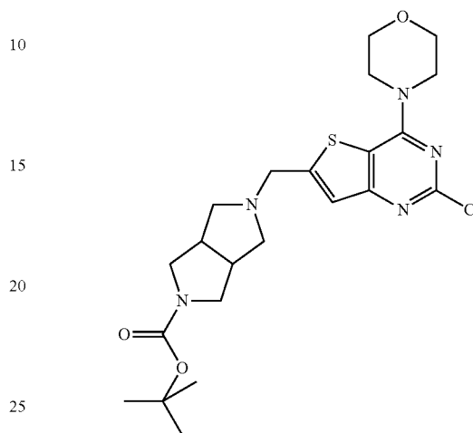
5-(2-Chloro-4-morpholin-4-yl-thieno[3,2-d]pyrimidin-6-ylmethyl)-hexahydro-pyrrolo[3,4-c]pyrrole-2-carboxylic acid tert-butyl ester
