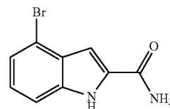
4-Bromo-1H-indole-2-carboxylic acid amide
