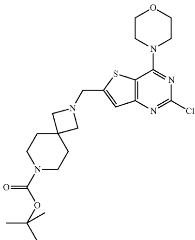
2-(2-Chloro-4-morpholin-4-yl-thieno[3,2-d]pyrimidin-6-ylmethyl)-2,7-diaza-spiro[3.5]nonane-7-carboxylic acid tert-butyl ester
