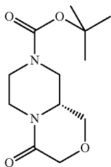
(R)-4-Oxo-hexahydro-pyrazino[2,1-c][1,4]oxazine-8-carboxylic acid tert-butyl ester
