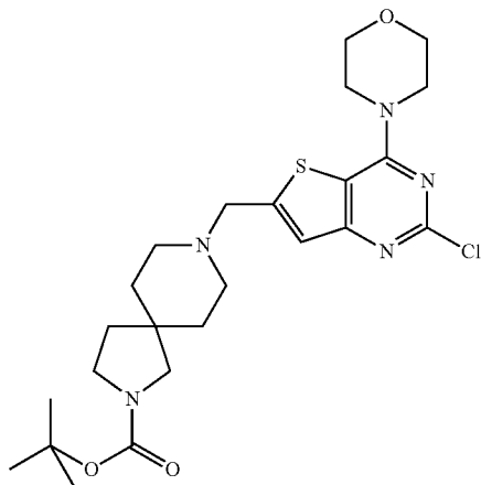
8-(2-Chloro-4-morpholin-4-yl-thieno[3,2-d]pyrimidin-6-ylmethyl)-2,8-diaza-spiro[4.5]decane-2-carboxylic acid tert-butyl ester
