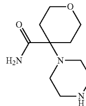
4-piperazin-1-yl-tetrahydro-pyran-4-carboxylic acid amide
