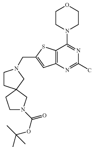
7-(2-Chloro-4-morpholin-4-yl-thieno[3,2-d]pyrimidin-6-ylmethyl)-2,7-diaza-spiro[4.4]nonane-2-carboxylic acid tert-butyl ester
