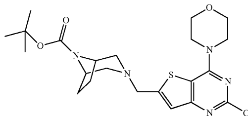
3-(2-Chloro-4-morpholin-4-yl-thieno[3,2-d]pyrimidin-6-ylmethyl)-3,8-diaza-bicyclo[3.2.1]octane-8-carboxylic acid tert-butyl ester
