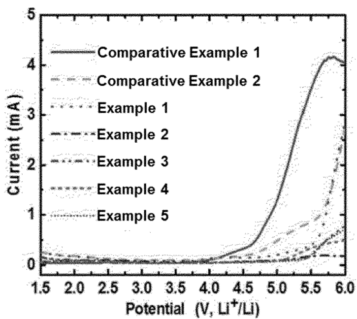
Graph for Voltage Stability
