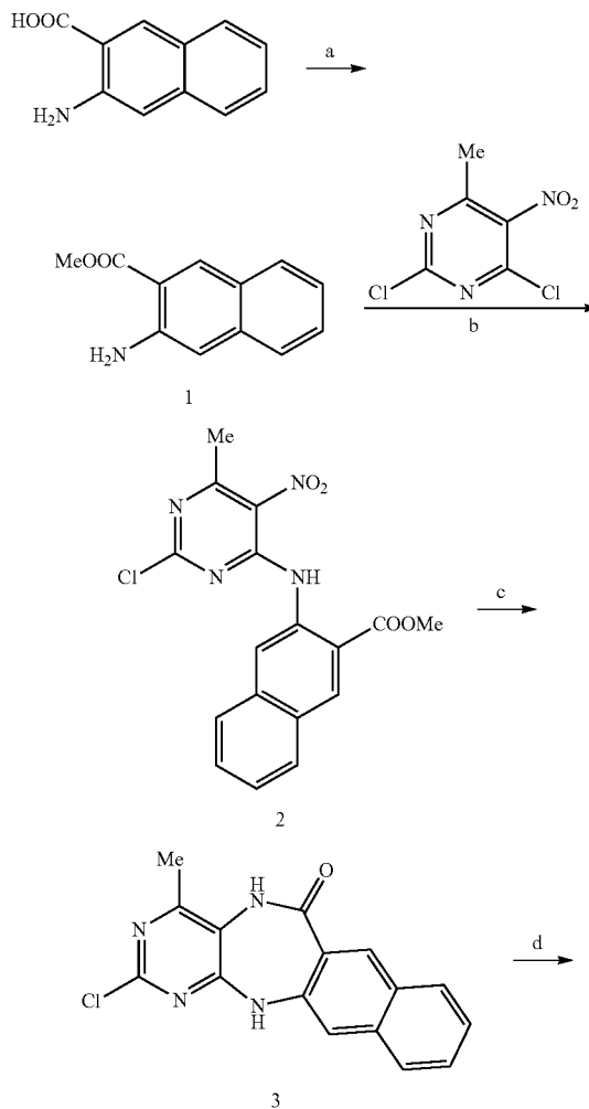
Scheme 8. Synthesis of 4,5,13-trimethyl-2- ((1-piperidin-4-yl)-1H-pyrazol-4-yl)amino)-5,13-dihydro- 6H-naphtho[2,3-e]pyrimido[5,4-b][1,4]diazepin-6-one (HTH-01-015) a
