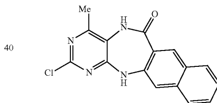
2-chloro-4-methyl-5,13-dihydro-6H-naphtho[2,3-e]pyrimido[5,4-b][1,4]diazepin-6-one
