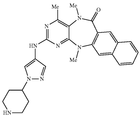
4,5,13-trimethyl-2-((1-(piperidin-4-yl)-1H-pyrazol-4-yl)amino)-5,13-dihydro-6H-naphtho[2,3-e]pyrimido[5,4-b][1,4]diazepin-6-one
