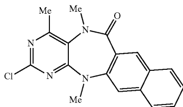
2-chloro-4,5,13-trimethyl-5,13-dihydro-6H-naphtho[2,3-e]pyrimido[5,4-b][1,4]diazepin-6-one
