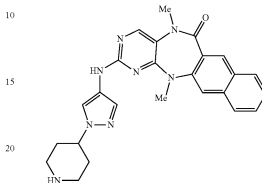
5,13-dimethyl-2-((1-(piperidin-4-yl)-1H-pyrazol-4-yl)amino)-5,13-dihydro-6H-naphtho[2,3-e]pyrimido[5,4-b][1,4]diazepin-6-one
