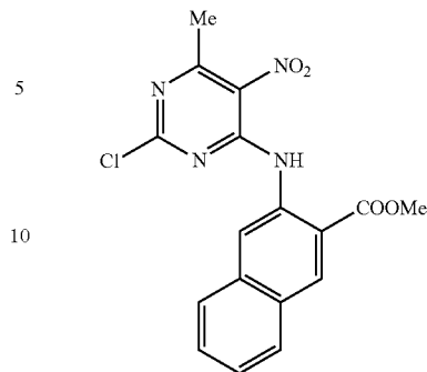
Methyl 3-((2-chloro-6-methyl-5-nitropyrimidin-4-yl)amino)-2-naphthoate
