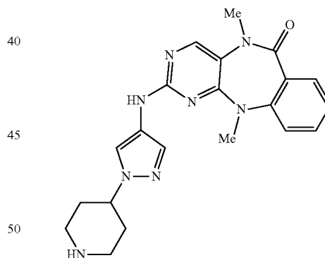
5,11-dimethyl-2-((1-(piperidin-4-yl)-1H-pyrazol-4-yl)amino)-5,11-dihydro-6H-benzo[e]pyrimido[5,4-b][1,4]diazepin-6-one
