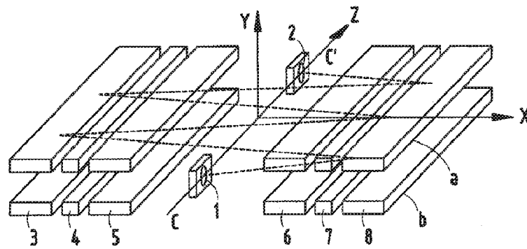
FIG. 2 (PRIOR ART)
