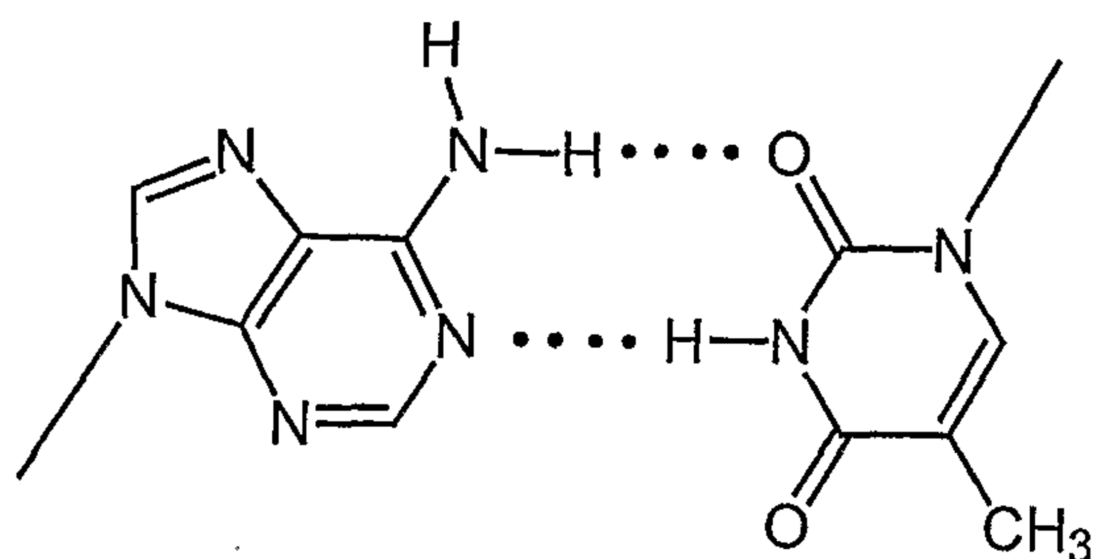
Reverse Watson Crick AT-Base Pair II parallel
