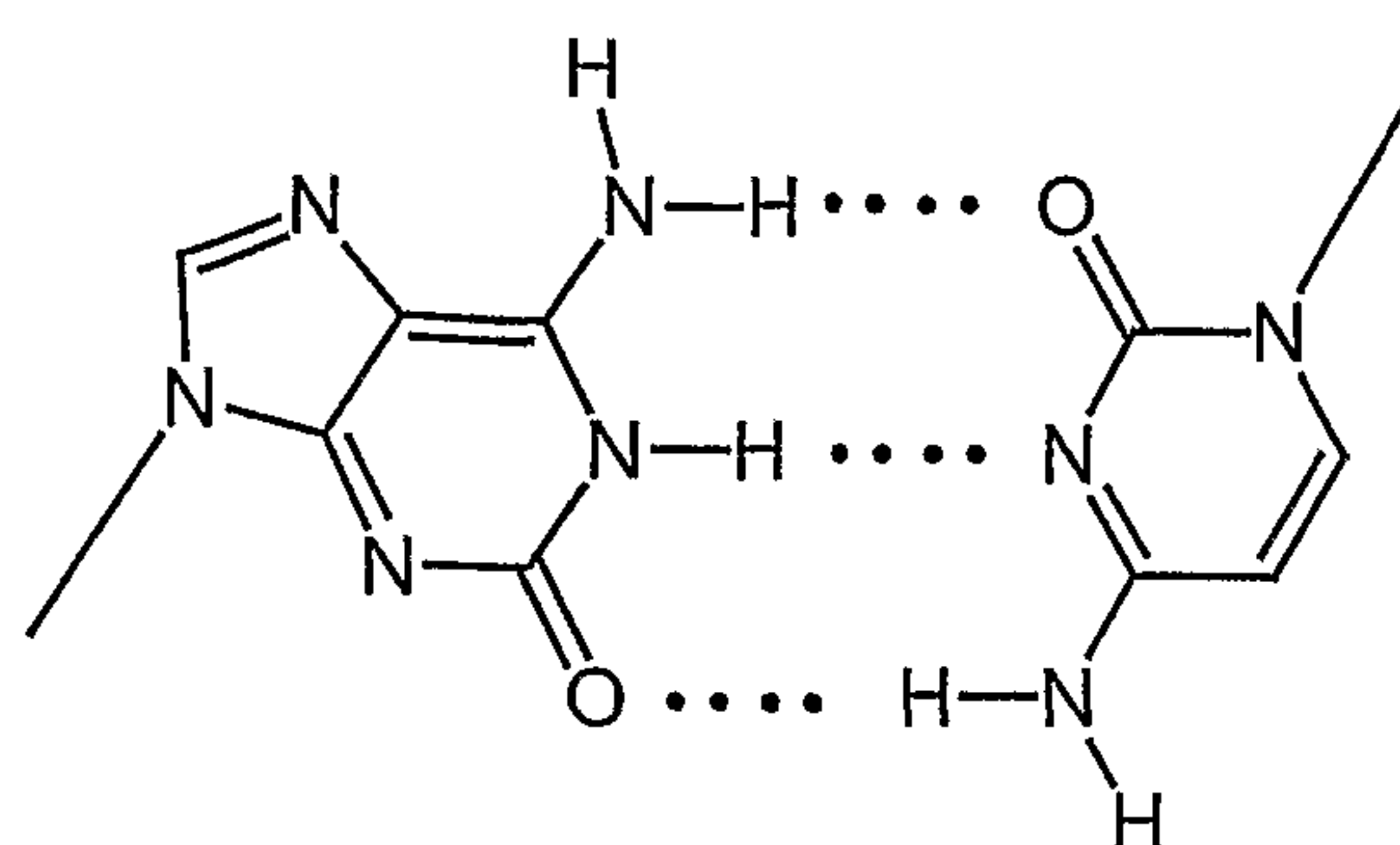
Reverse Watson Crick iGC-Base Pair VIII parallel
