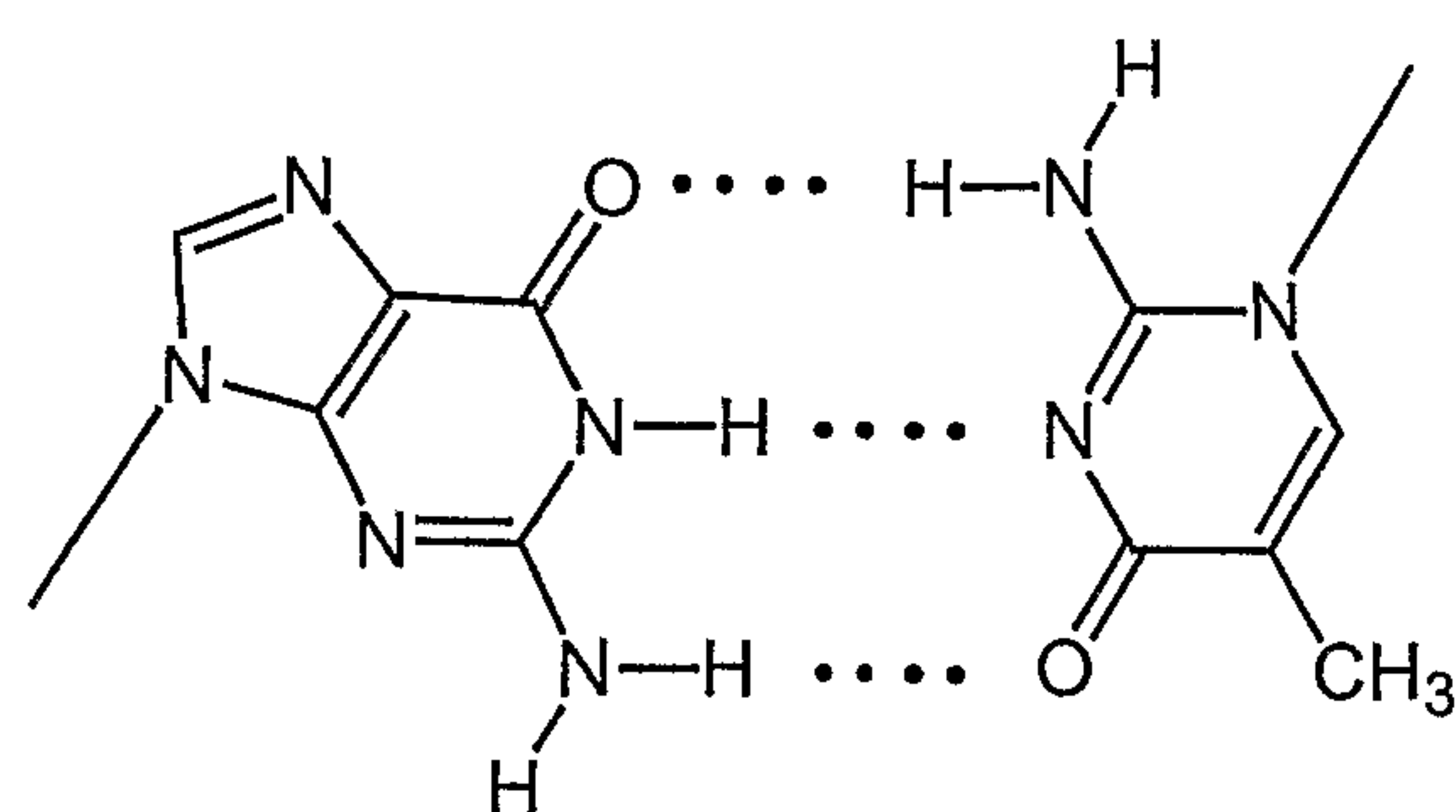
Reverse Watson Crick G me iC-Base Pair X parallel
