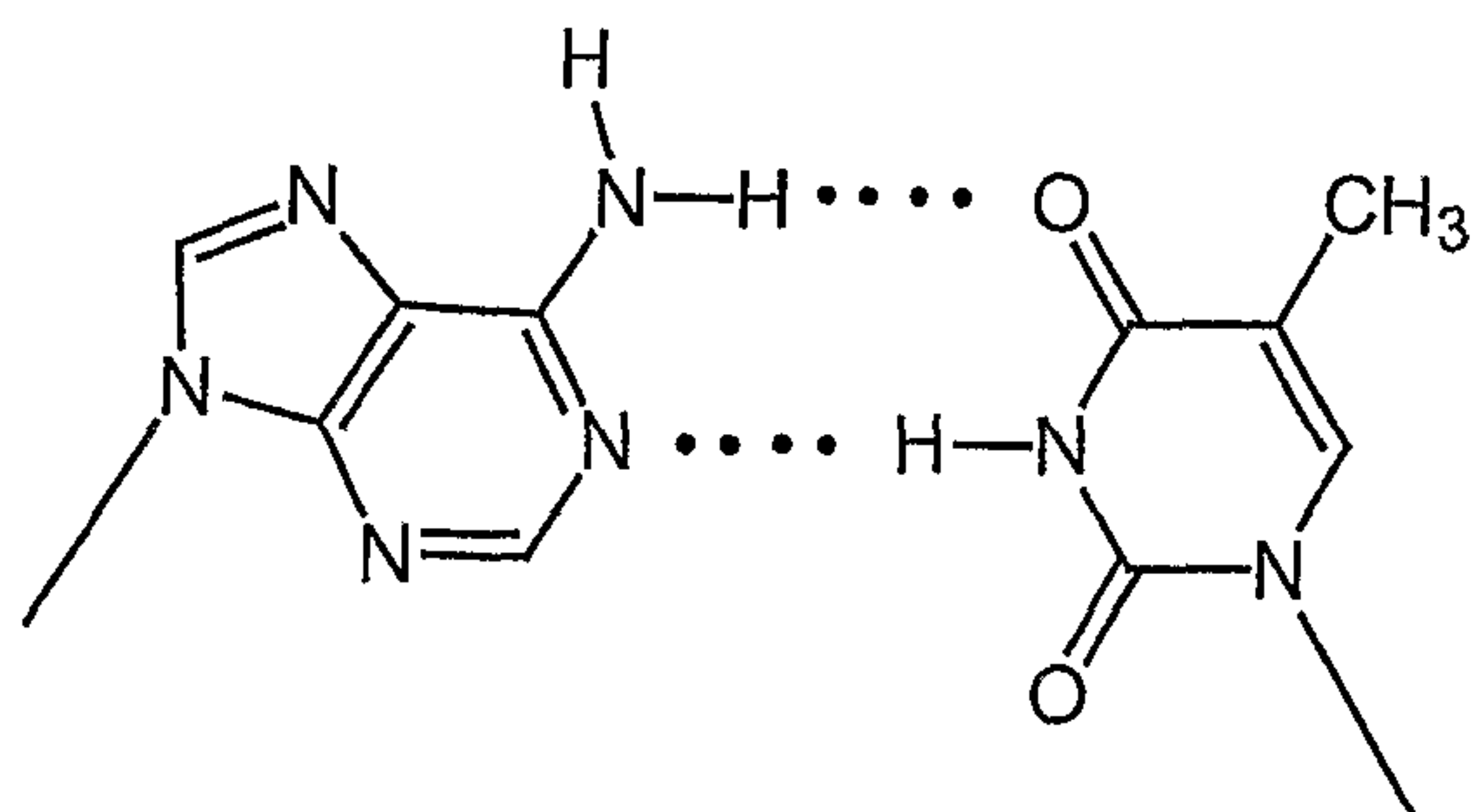
Watson Crick AT-Base Pair I antiparallel
