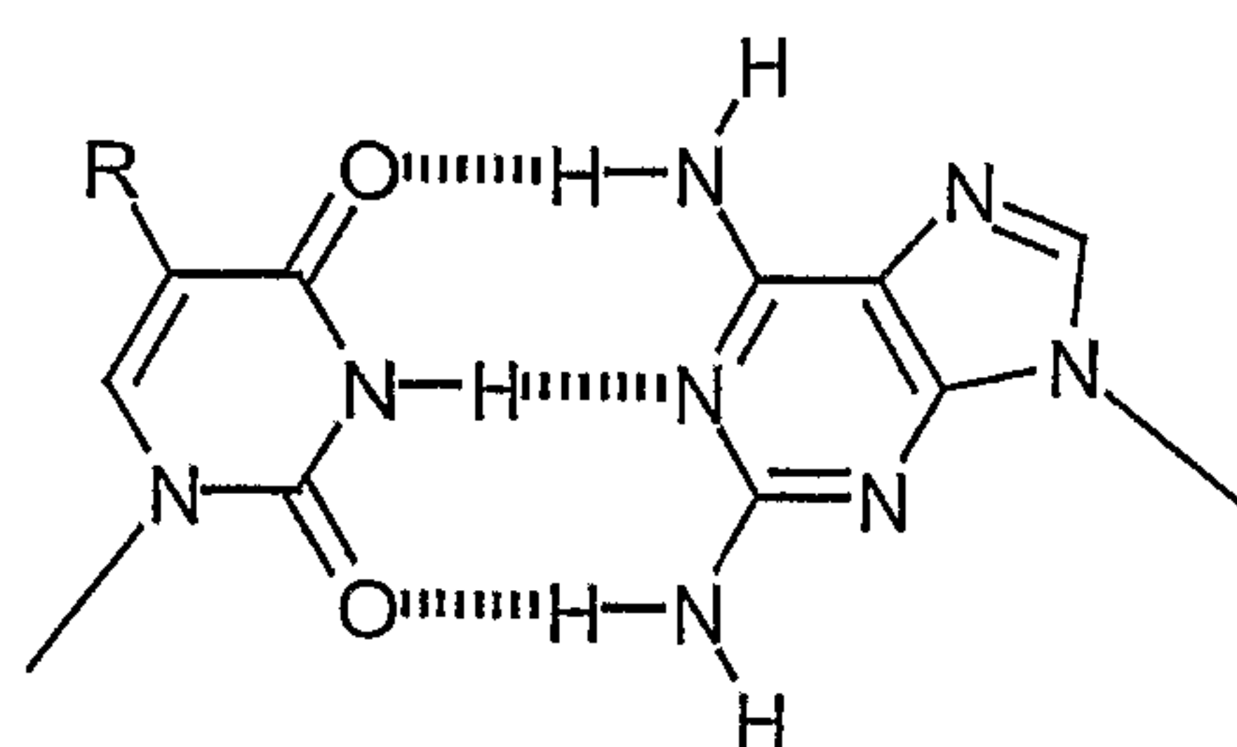
base pair IIIa : R = H IIIb : R = Br IIIc : R = I
