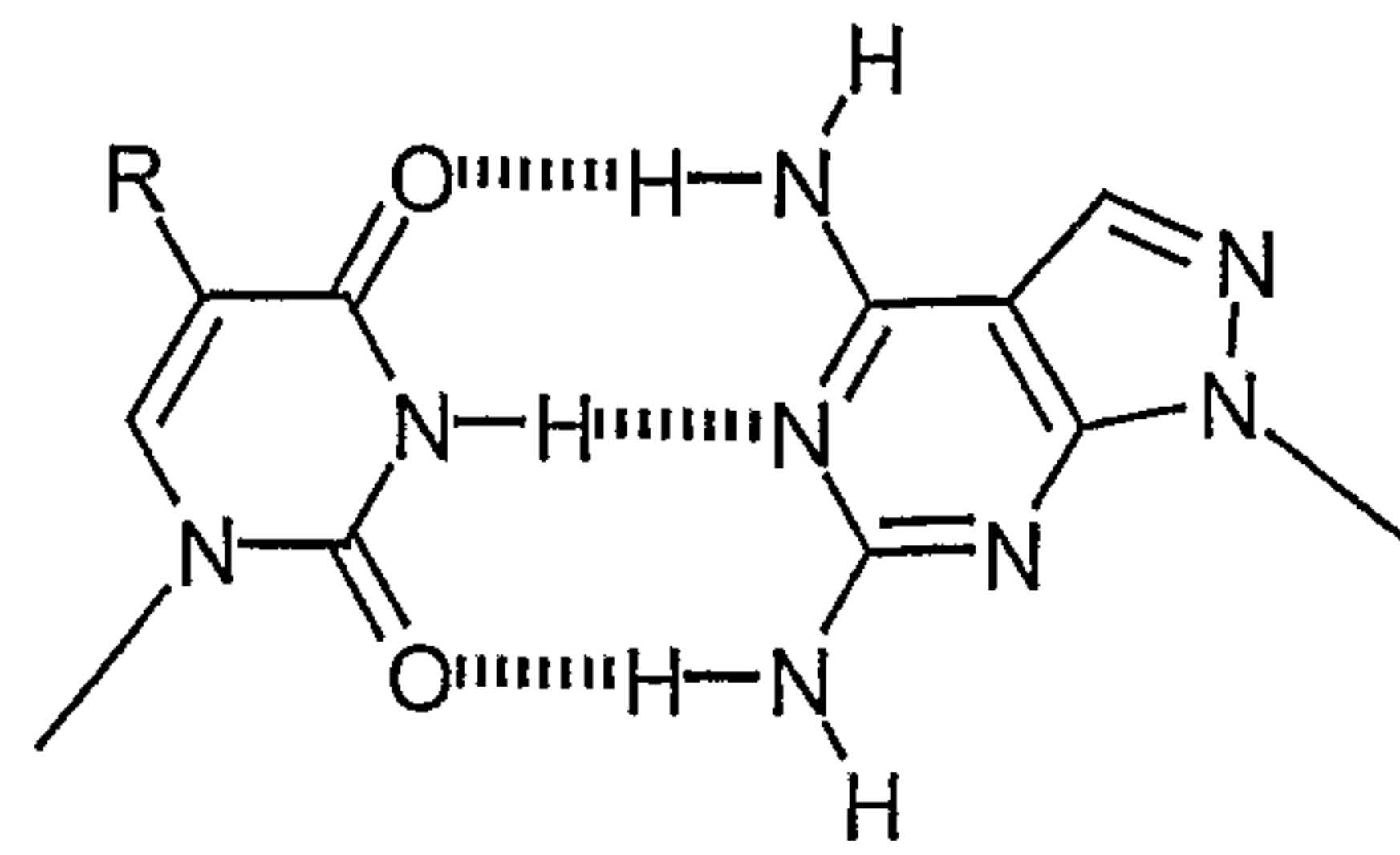
base pair IVa : R = H IVb : R = Br IVc : R = I
