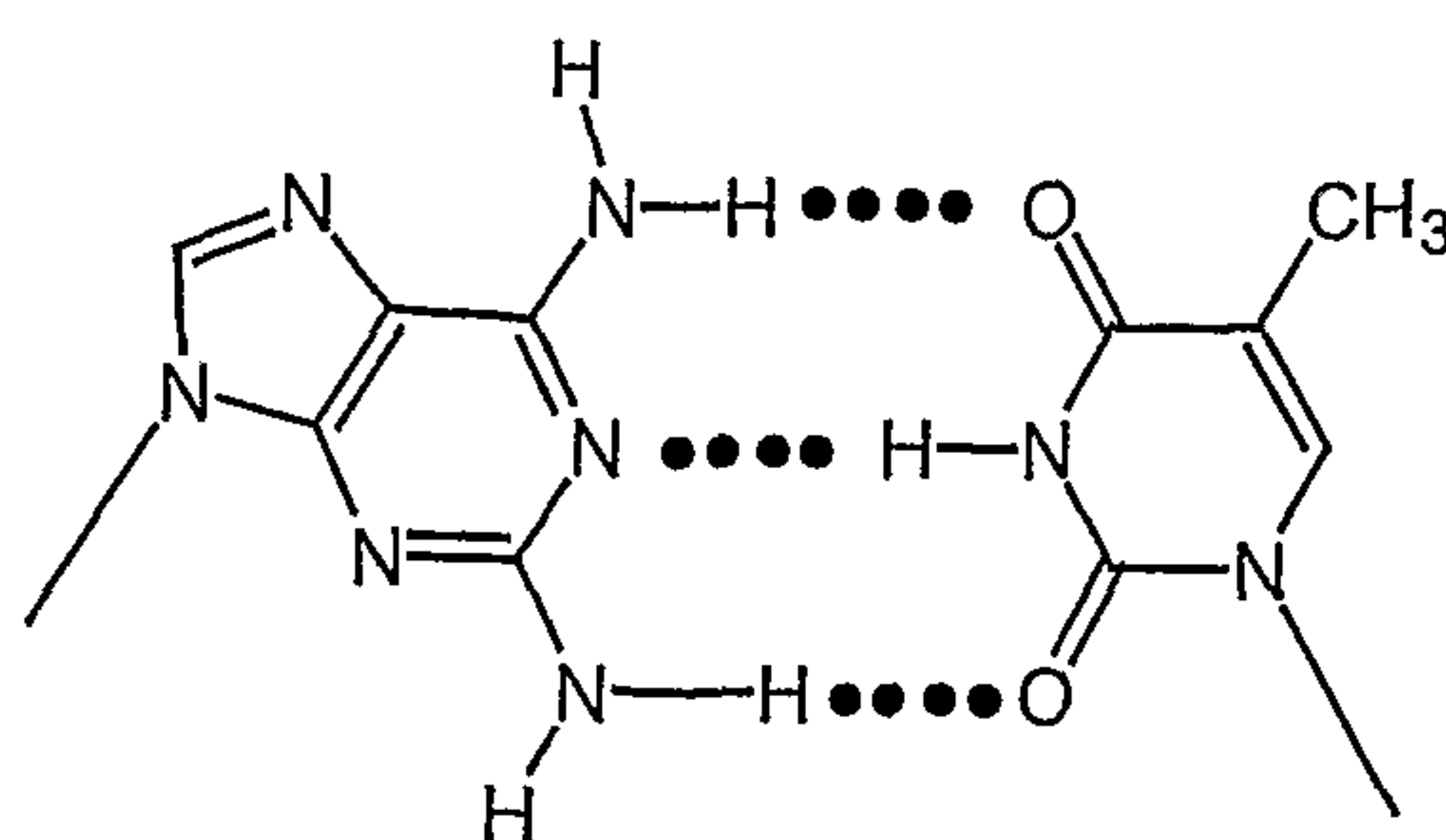
Watson Crick Base Pair II
