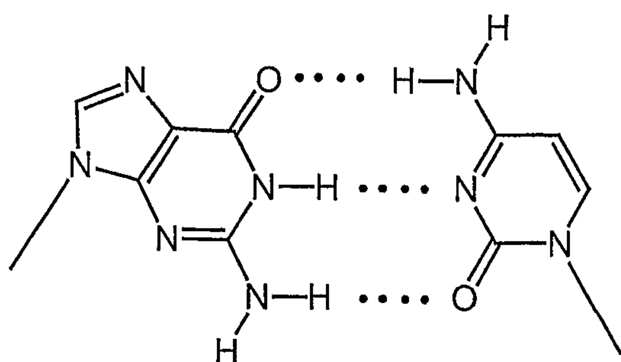
Watson Crick GC-Base Pair VII antiparallel
