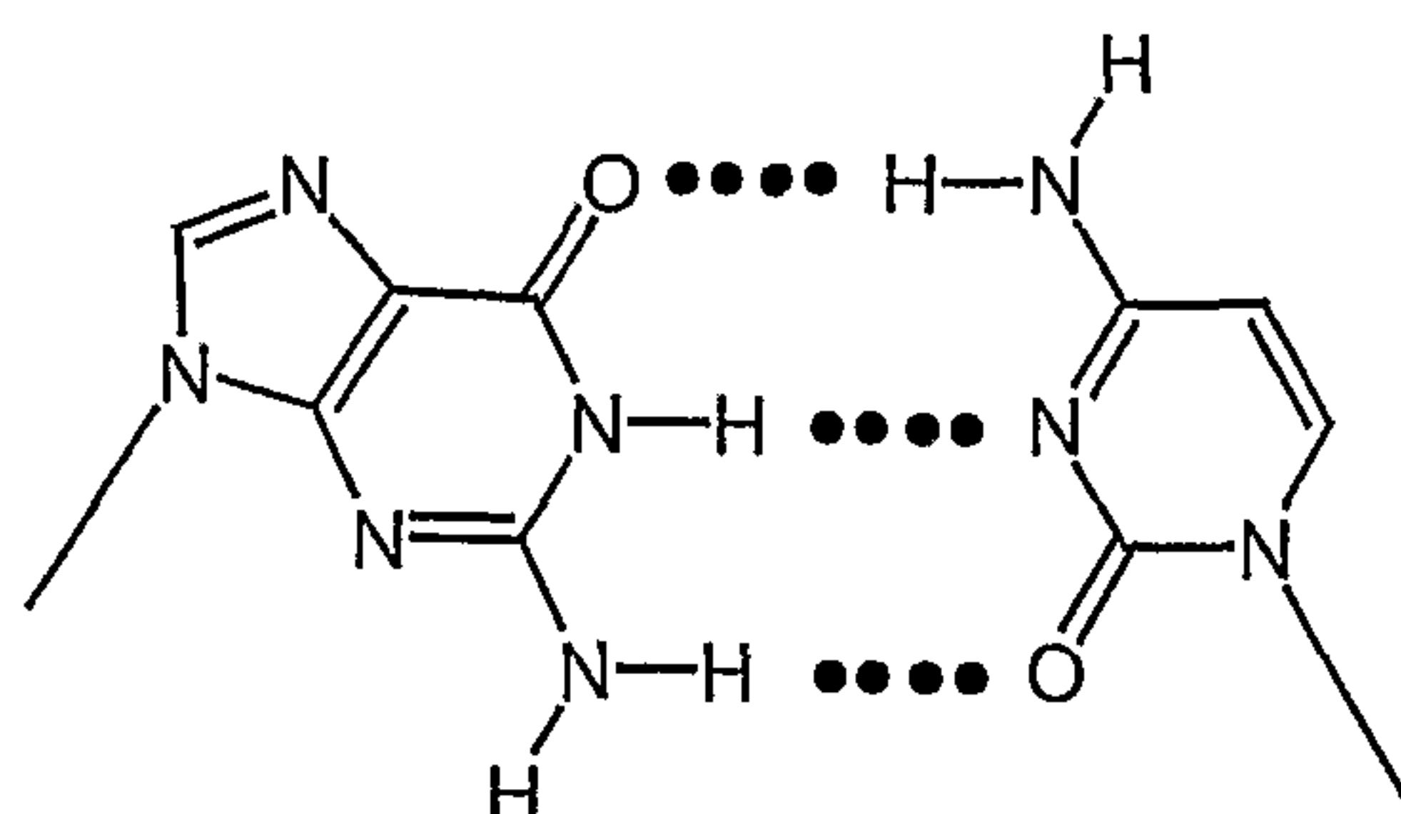
Watson Crick Base Pair III
