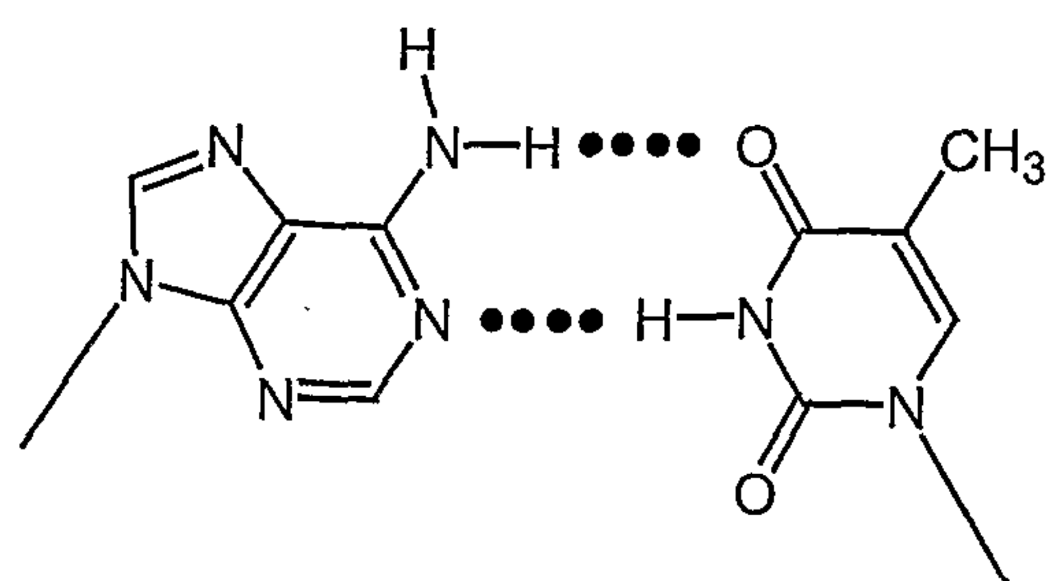
Watson Crick Base Pair I
