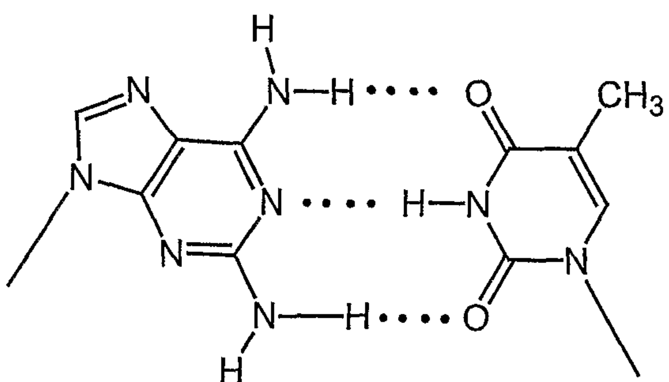
Watson Crick n 2 AT-Base Pair III antiparallel
