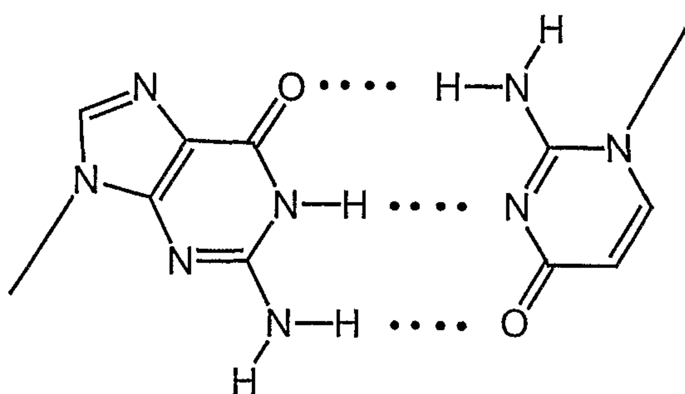
Reverse Watson Crick GiC-Base Pair IX parallel
