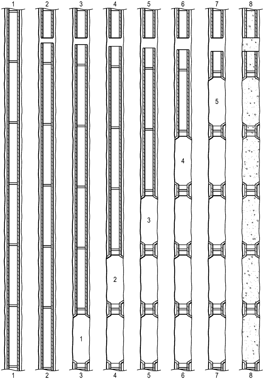
CASING EXPANSION - EARTH BARRIER P & A
