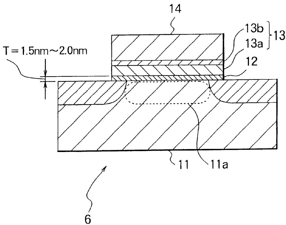
SECTIONAL VIEW OF CONVENTIONAL MONOS TYPE NONVOLATILE MEMORY DEVICE
