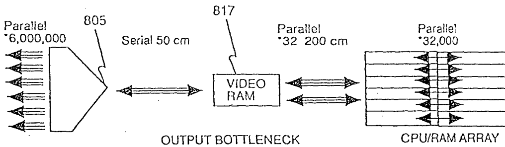
Typical Classic Massively Parallel System (Data Flow)
