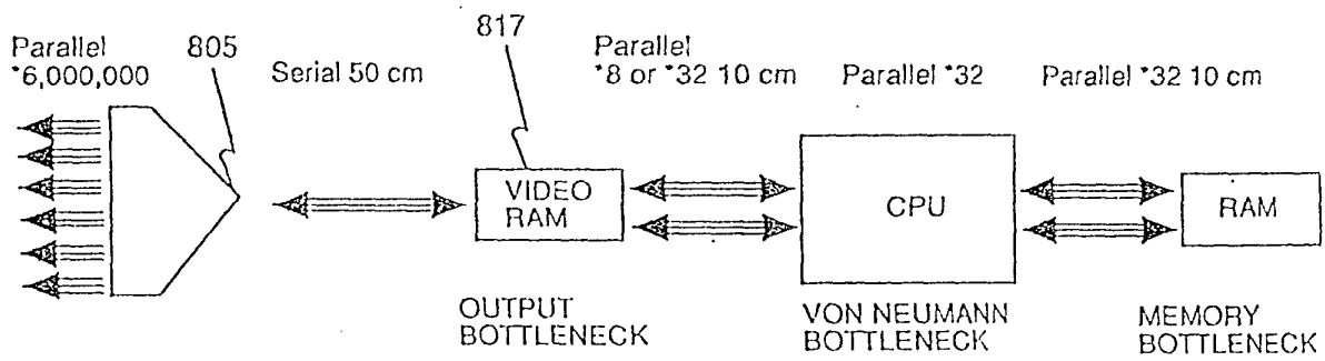
Typical Classic Architecture System (Data Flow)
