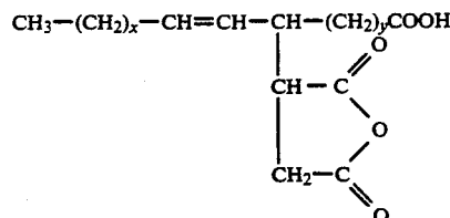
Maleinized Rosin
