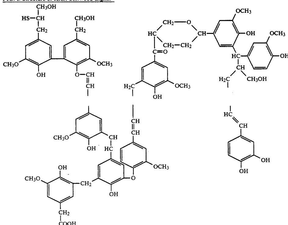
FIG. 1. Structure of Kraft Softwood Lignin
