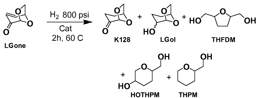
Reaction Scheme A
