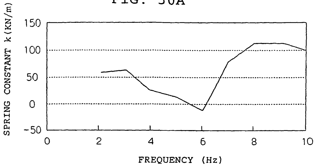
FREQUENCY CHARACTERISTIC OF SPRING CONSTANT
