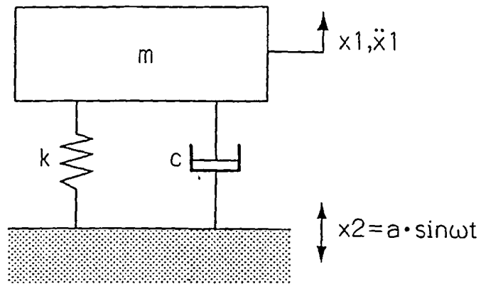
VIBRATION MODEL AT 1 DEGREE OF FREEDOM
