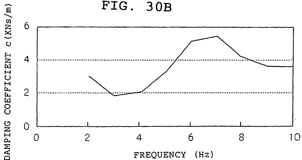
FREQUENCY CHARACTERISTIC OF DAMPING COEFFICIENT
