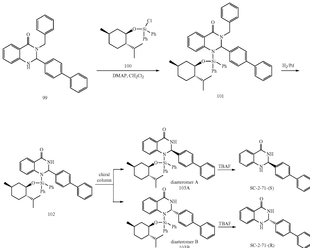
Scheme 12. Chiral resolution of SC-2-71.
