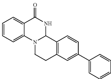
Rigid Analogues (amine)
