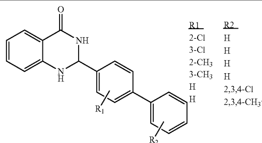
Aryl Substitution (Biphenyl)
