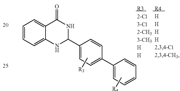
Aryl Substitution (Biphenyl)
