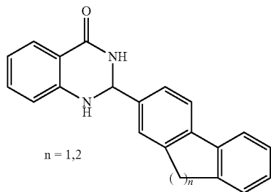
Biphenyl Rigid Analogues
