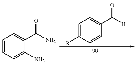
Scheme 1 Synthetic route for SC-2-71 and analogues.
