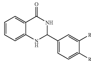
Scheme 1 Synthetic route for SC-2-71 and analogues.
