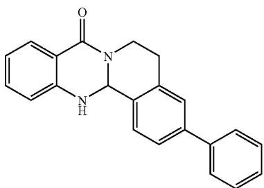
Rigid Analogues (amide linked)
