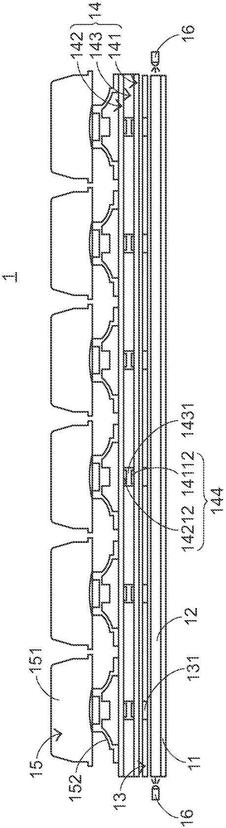
FIG.1 PRIOR ART
