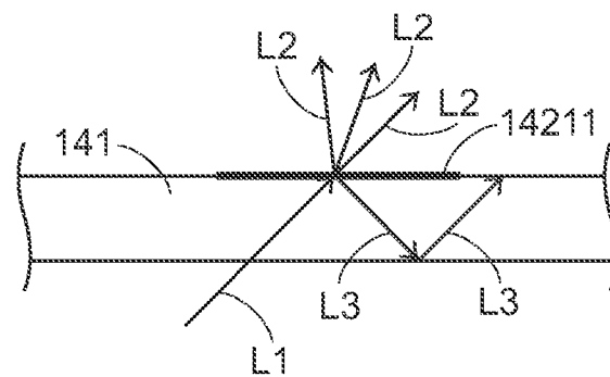
FIG. 3 PRIOR ART
