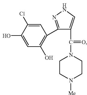
1-[[3-(5-chloro-2,4-dihydroxyphenyl)-1H-pyrazol-4-yl]carbonyl]-4-methyl-piperazine
