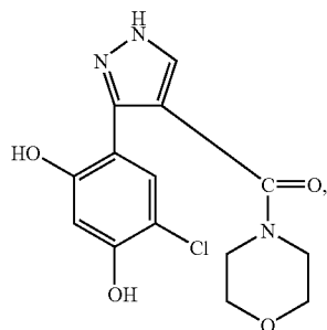
1-[[3-(5-chloro-2,4-dihydroxyphenyl)-1H-pyrazol-4-yl]carbonyl]-4-methyl-piperazine
