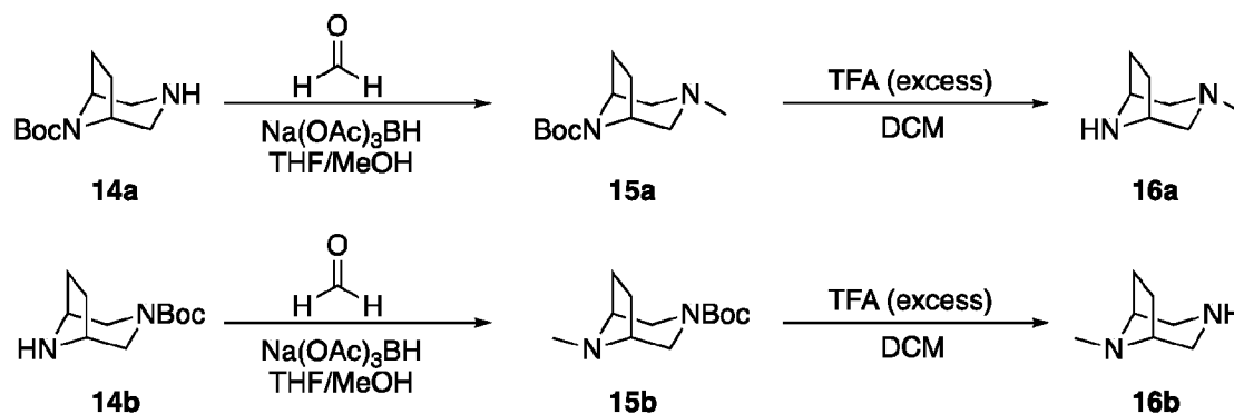
Scheme 14: General synthetic scheme for compounds 16a and 16b .
