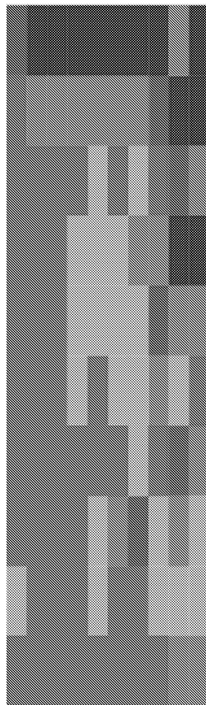
Inhibition profile of Compound 1 and analogs
