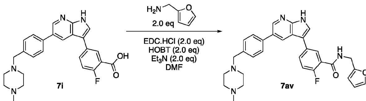
Scheme 3: Synthesis of compound 7av.
