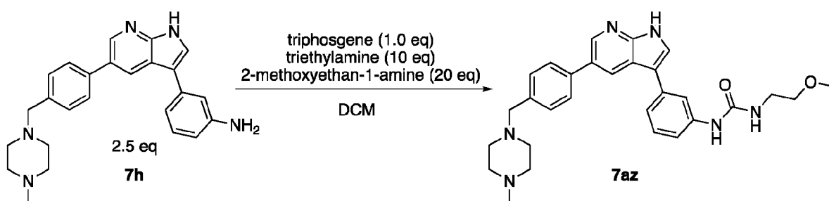
Scheme 7: Synthesis of compound 7az.
