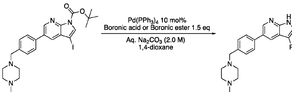
Scheme 2: General synthetic scheme for Suzuki coupling and in situ deprotection.
