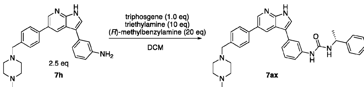
Scheme 5: Synthesis of compound 7ax.
