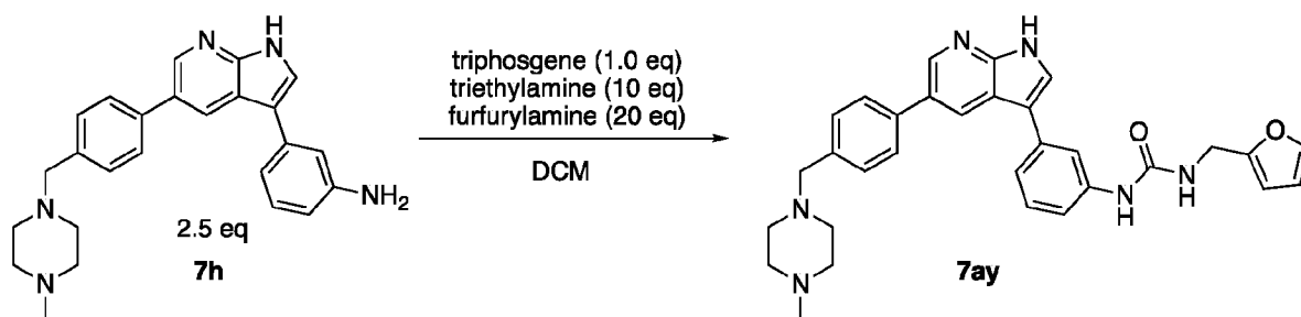
Scheme 6: Synthesis of compound 7ay.
