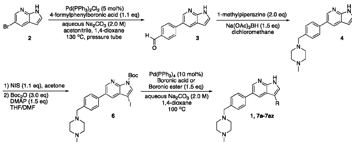
Scheme 1: General synthetic scheme for compounds 1 and 7a – 7az .
