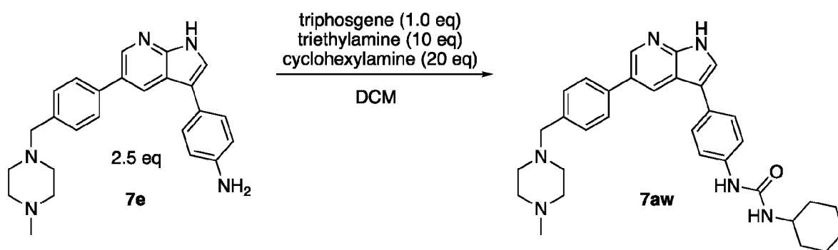
Scheme 4: Synthesis of compound 7aw.
