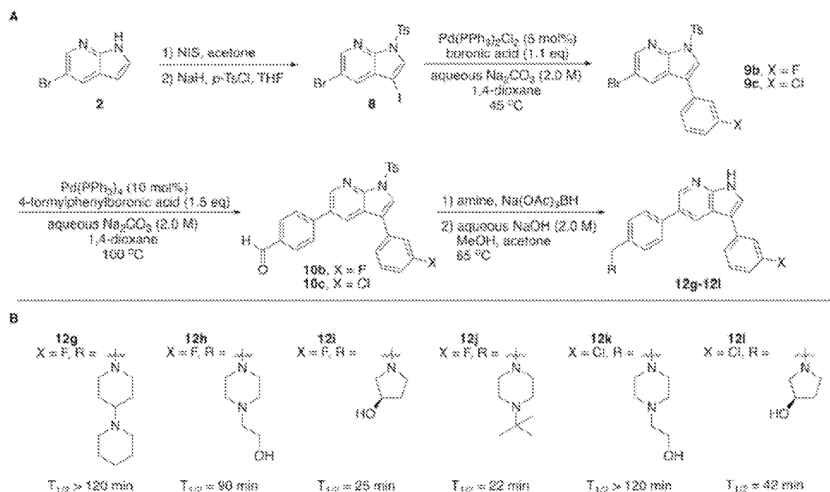
Scheme 12: (A) Synthesis of analogs 12g – 12l ; (B) Structures of analogs 12g – 12l and their half-lives in mouse liver microsomes.
