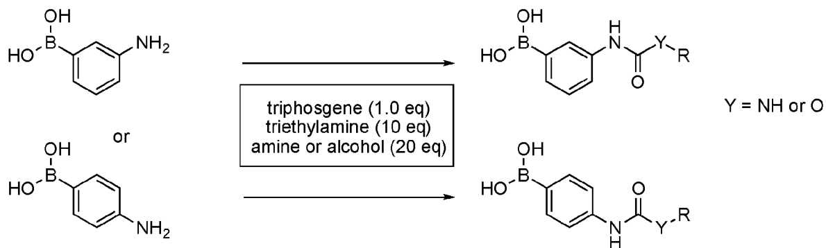
Scheme 13: General synthetic scheme for compounds 13a – 13e .
