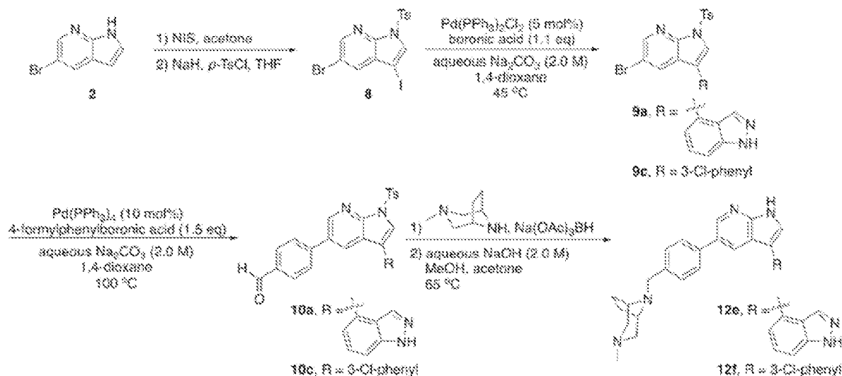
Scheme 11: Synthesis of compounds 12e and 12f .
