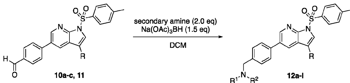
Scheme 10: General synthetic scheme for compounds 12a – 12l .
