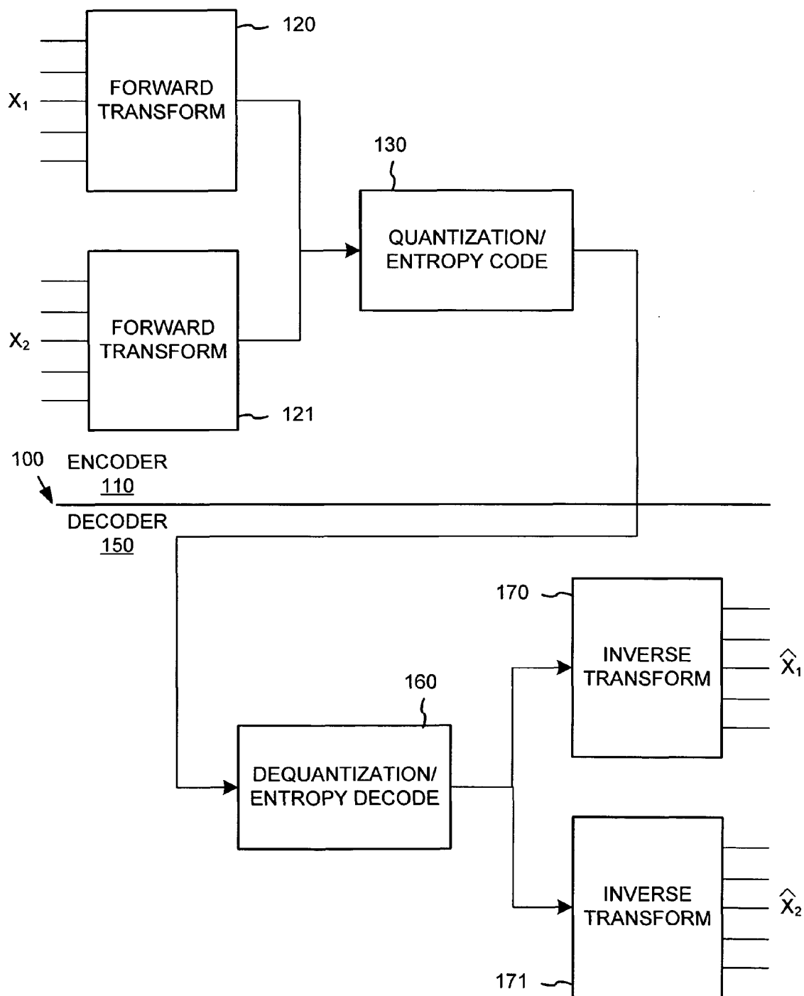
Figure 1 Prior Art
