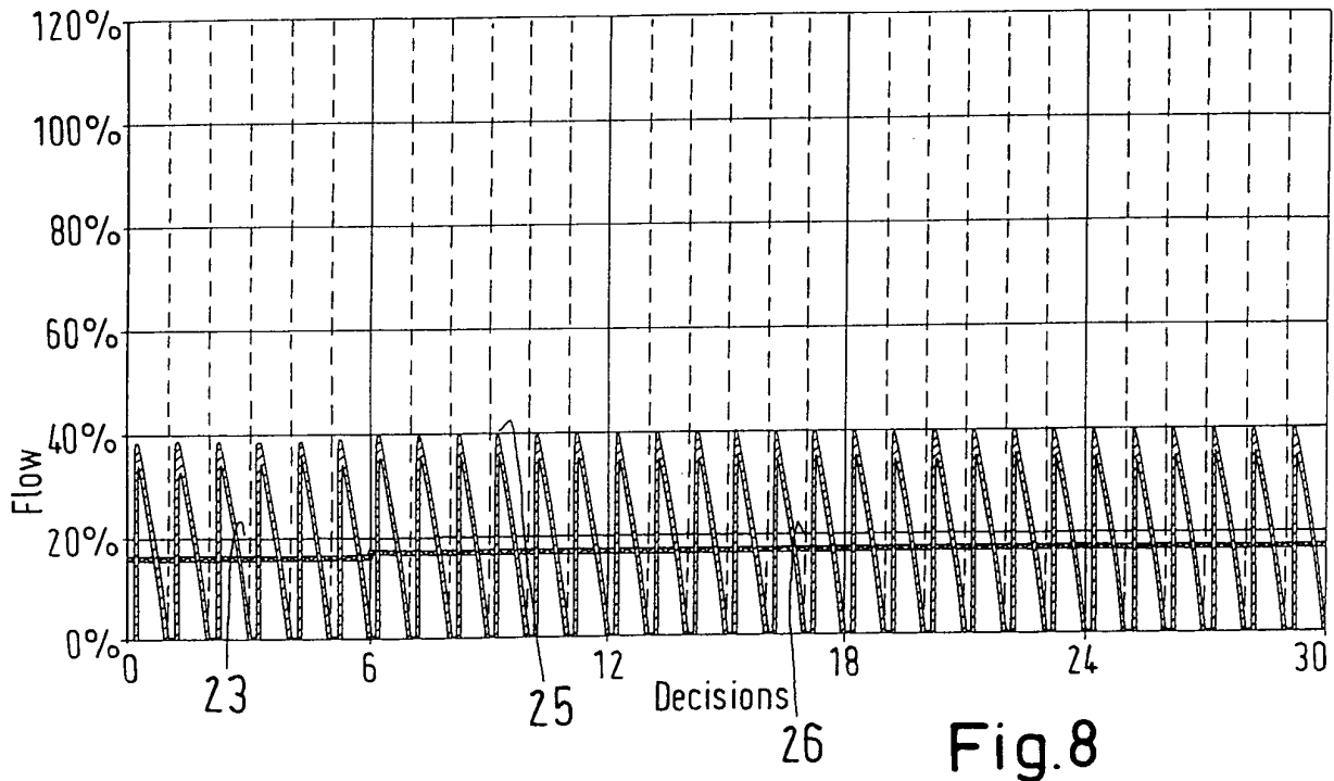
Simulated Flow
