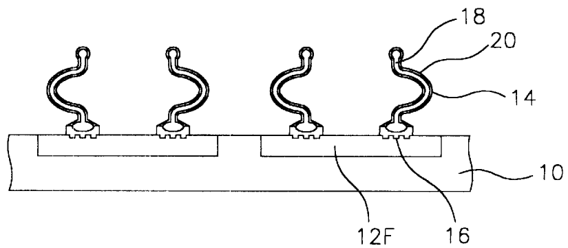
FIGURE 2C (PRIOR ART)
