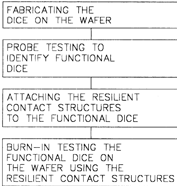
FIGURE 1 (PRIOR ART)
