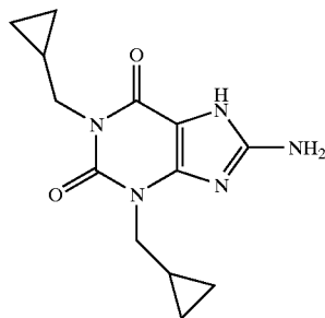
Cipamfylline
