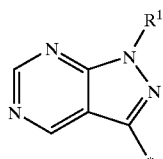
1H-pyrazolo[3,4-d]- pyrimidinyl
