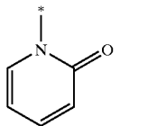
pyrid-2-on-1-yl
