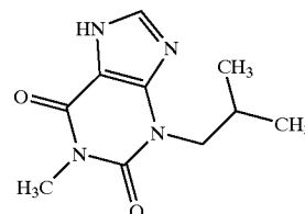
IBMX
