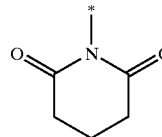
glutarimid-1-yl
