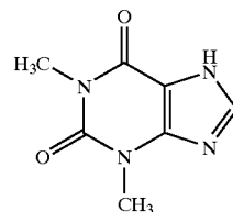
Theophylline
