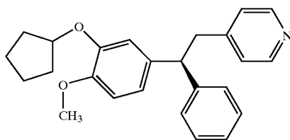
CT-1731
