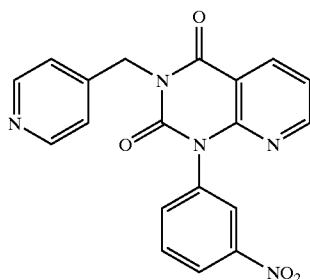
RS-25,344
