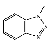
benzothiazolyl
