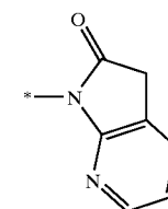
pyrrolo[4,5-b]pyridin- 3-on-2-yl
