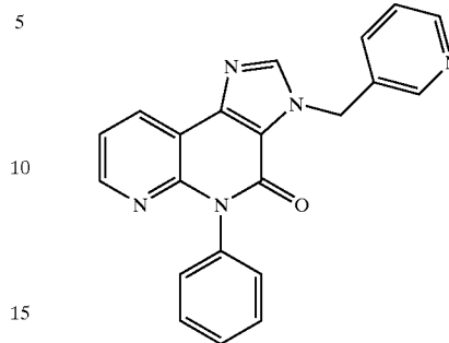
KF19514
