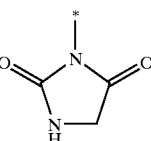
imidazolidin-2,4-dion-1-yl
