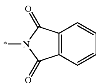
pyrrolo[3,4-b]pyridin- 5,7-dion-6-yl
