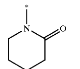
piperid-2-on-1-yl
