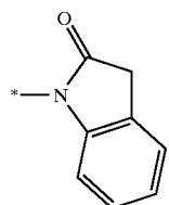
1,3-dihydro-indol-2-on-1-yl
