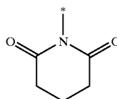
glutarimid-1-yl
