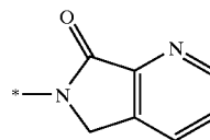
pyrrolo[3,4-b]pyridin- 7-on-6-yl
