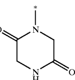
piperazin-2,5-dion-1-yl
