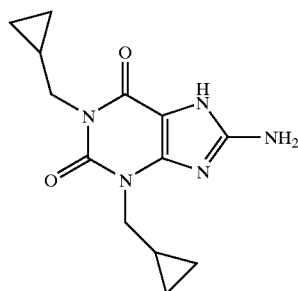
Cipamfylline (BRL-61,063)
