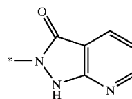
1H-pyrazolo[4,5- e]pyridin-4-on-2-yl
