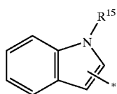
indoyl
