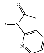
pyrrolo[4,5-b]pyridin-3-on-2-yl
