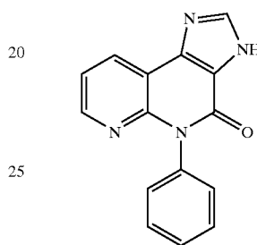
KF17625
