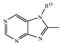
1H-purinyl
