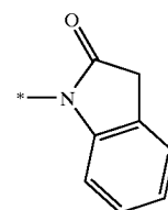
1,3-dihydro-indol-2- on-1-yl
