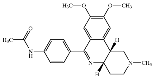
Benafentrine
