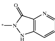
1H-pyrazolo[4,5-e]pyridin-7-on-2-yl
