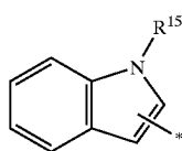
indoyl
