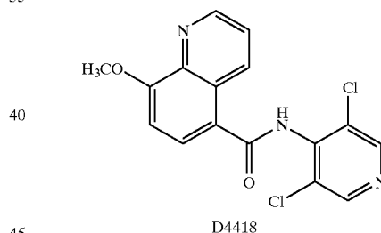
D4418
