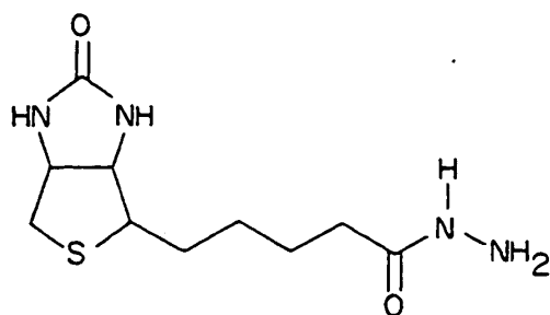
BIOTIN HYDRAZIDE
