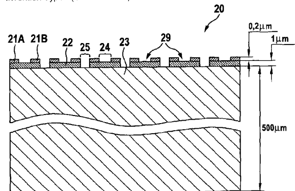
Invention Type I (Cross section)
