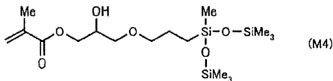
[Chemical Formula 9]
