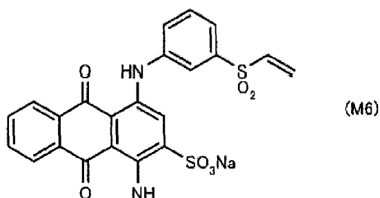
[Chemical Formula 11]
