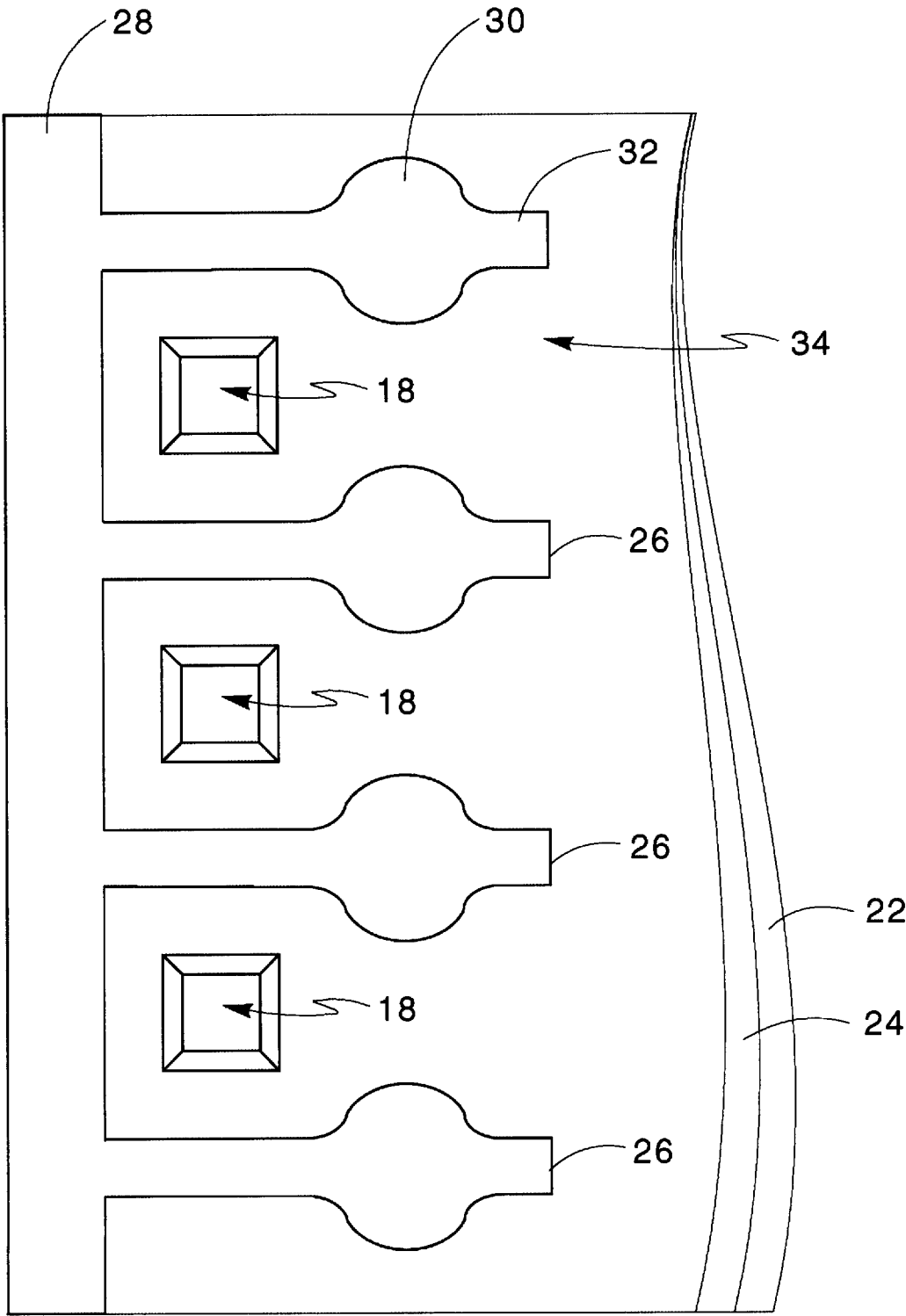
Top View of Base Plate 22 of Fig. 1
